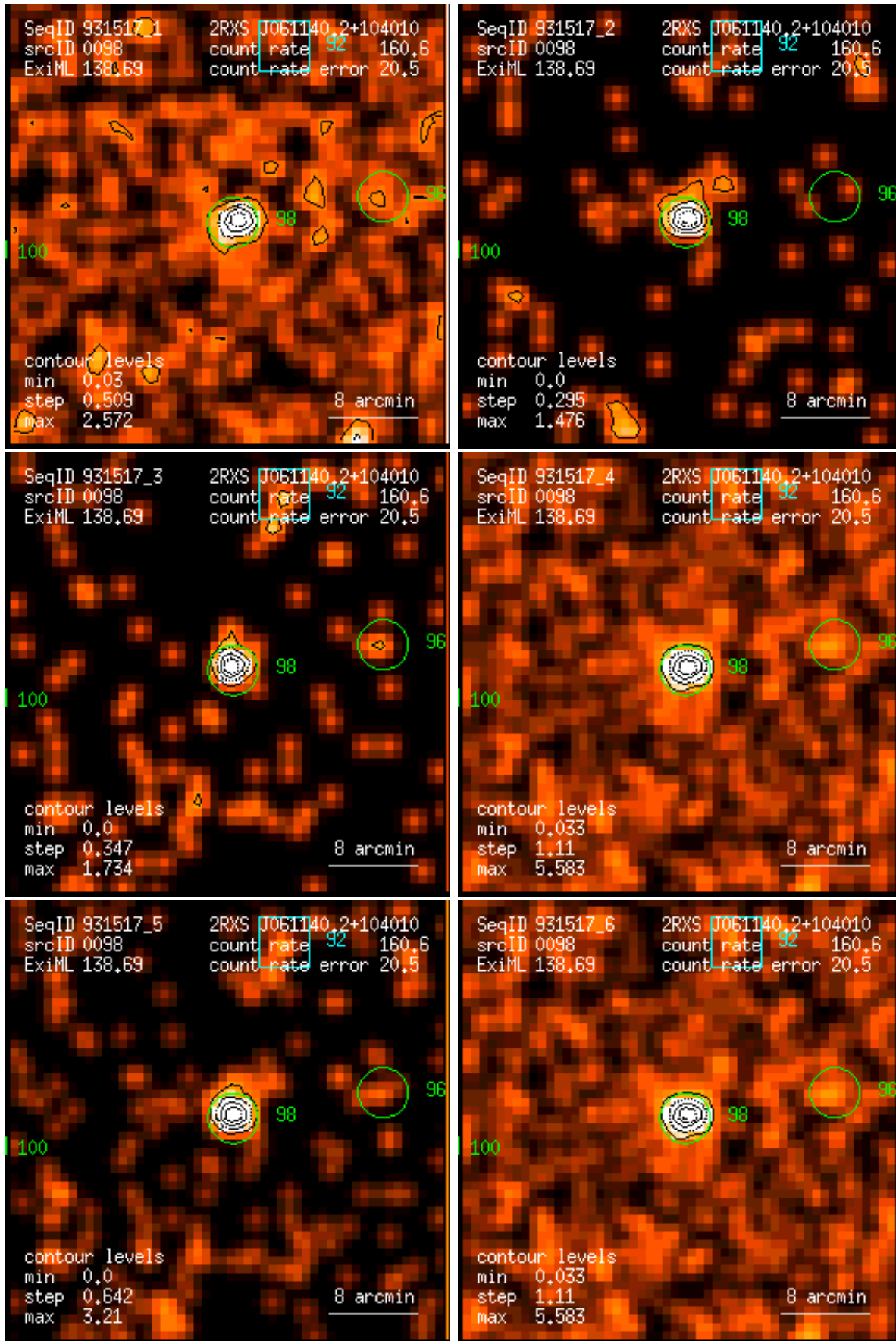
Figure 98: RASS 931517: detection 0098: band rate images, Gaussian filter: (1) PSPC channels 11 – 41, (2) 52 – 90, (3) 91 – 201, (4) 11 – 235, (5) 52 – 201, (6) 11 – 201. Broad band rates in counts/ks. Band rate contour levels in counts/ks/arcmin 2 .
