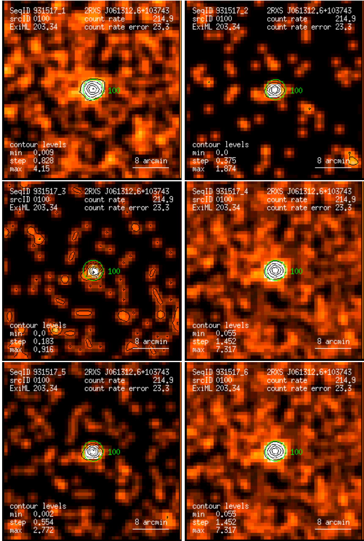
Figure 100: RASS 931517: detection 0100: band rate images, Gaussian filter: (1) PSPC channels 11 – 41, (2) 52 – 90, (3) 91 – 201, (4) 11 – 235, (5) 52 – 201, (6) 11 – 201. Broad band rates in counts/ks. Band rate contour levels in counts/ks/arcmin 2 .
