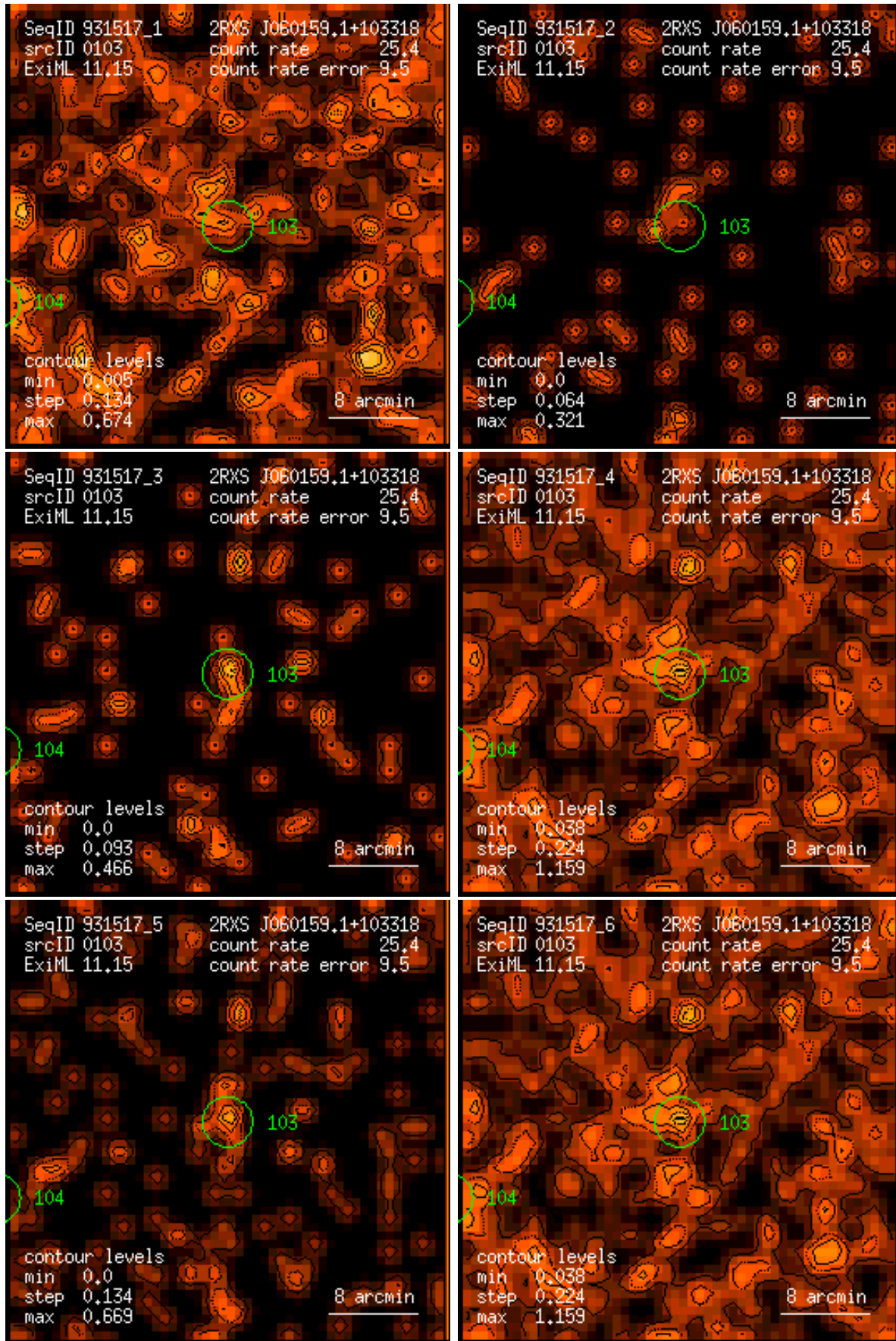
Figure 103: RASS 931517: detection 0103: band rate images, Gaussian filter: (1) PSPC channels 11 – 41, (2) 52 – 90, (3) 91 – 201, (4) 11 – 235, (5) 52 – 201, (6) 11 – 201. Broad band rates in counts/ks. Band rate contour levels in counts/ks/arcmin 2 .
