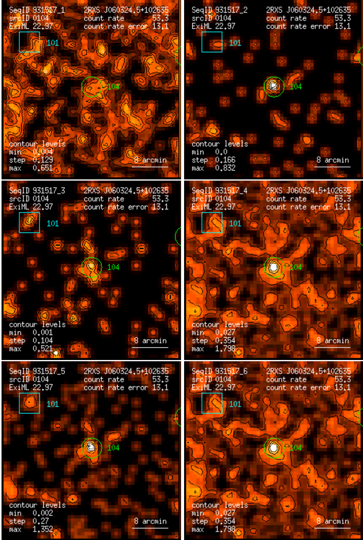
Figure 104: RASS 931517: detection 0104: band rate images, Gaussian filter: (1) PSPC channels 11 – 41, (2) 52 – 90, (3) 91 – 201, (4) 11 – 235, (5) 52 – 201, (6) 11 – 201. Broad band rates in counts/ks. Band rate contour levels in counts/ks/arcmin 2 .
