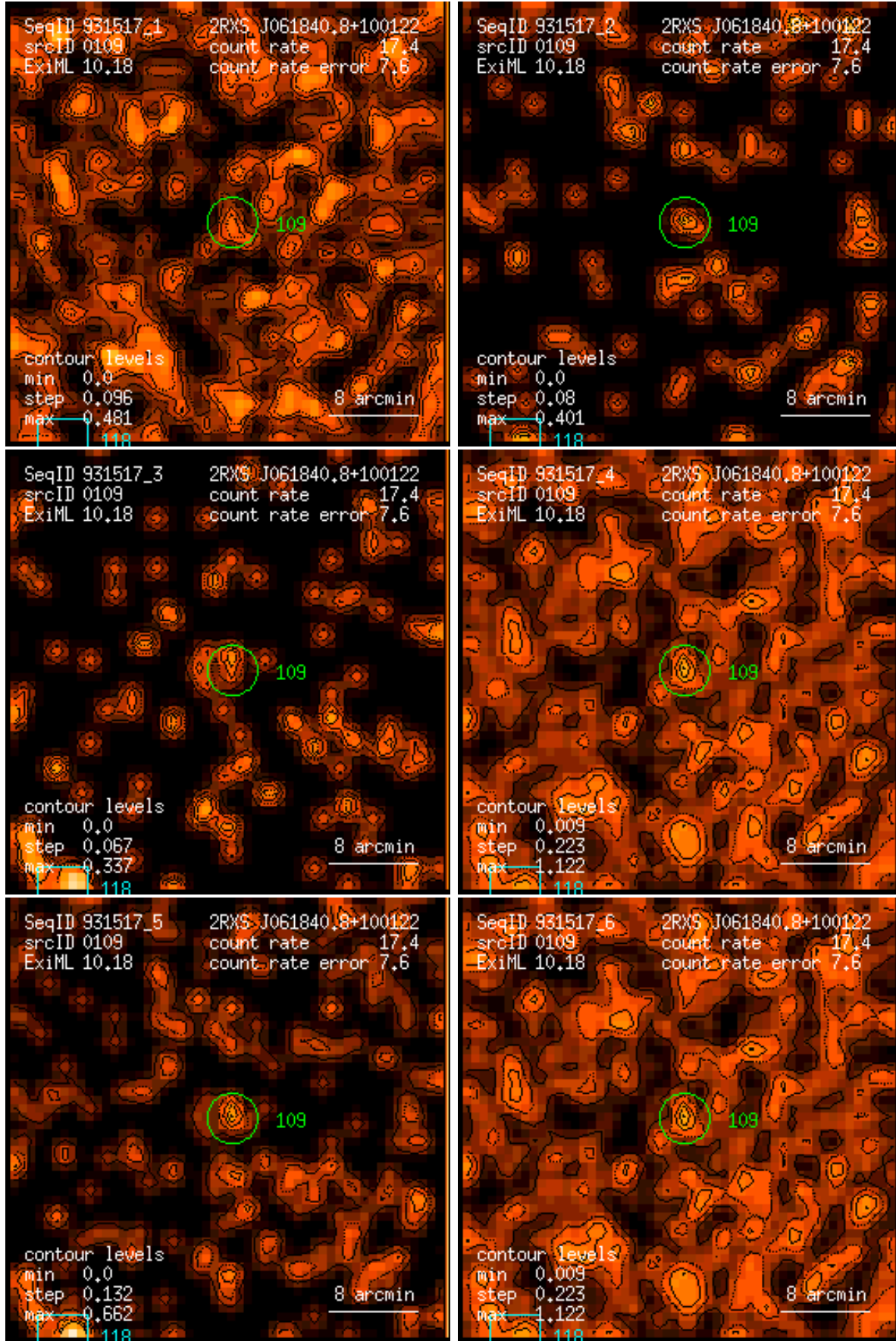
Figure 109: RASS 931517: detection 0109: band rate images, Gaussian filter: (1) PSPC channels 11 – 41, (2) 52 – 90, (3) 91 – 201, (4) 11 – 235, (5) 52 – 201, (6) 11 – 201. Broad band rates in counts/ks. Band rate contour levels in counts/ks/arcmin 2 .
