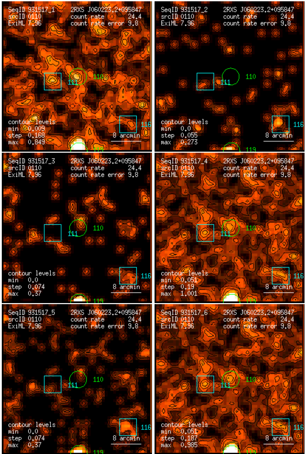
Figure 110: RASS 931517: detection 0110: band rate images, Gaussian filter: (1) PSPC channels 11 – 41, (2) 52 – 90, (3) 91 – 201, (4) 11 – 235, (5) 52 – 201, (6) 11 – 201. Broad band rates in counts/ks. Band rate contour levels in counts/ks/arcmin 2 .
