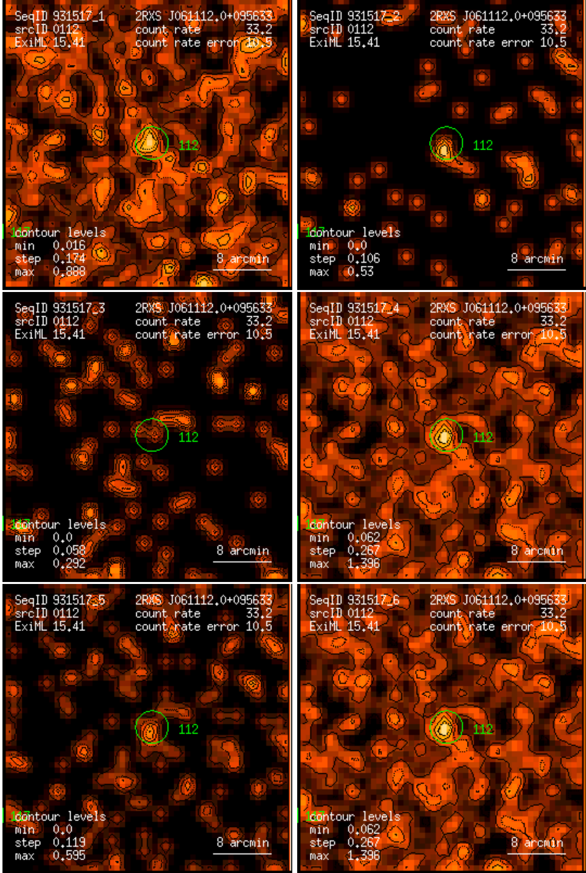
Figure 112: RASS 931517: detection 0112: band rate images, Gaussian filter: (1) PSPC channels 11 – 41, (2) 52 – 90, (3) 91 – 201, (4) 11 – 235, (5) 52 – 201, (6) 11 – 201. Broad band rates in counts/ks. Band rate contour levels in counts/ks/arcmin 2 .
