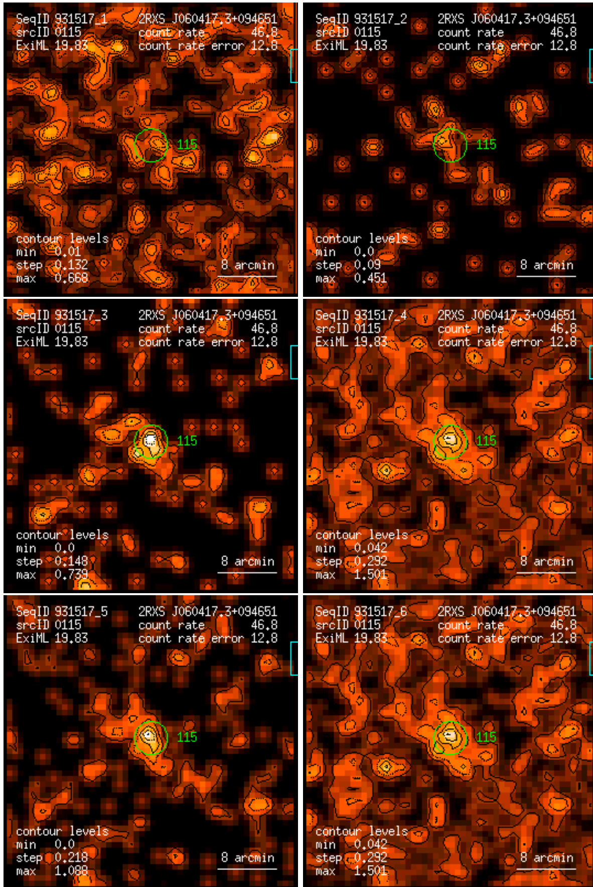
Figure 115: RASS 931517: detection 0115: band rate images, Gaussian filter: (1) PSPC channels 11 – 41, (2) 52 – 90, (3) 91 – 201, (4) 11 – 235, (5) 52 – 201, (6) 11 – 201. Broad band rates in counts/ks. Band rate contour levels in counts/ks/arcmin 2 .
