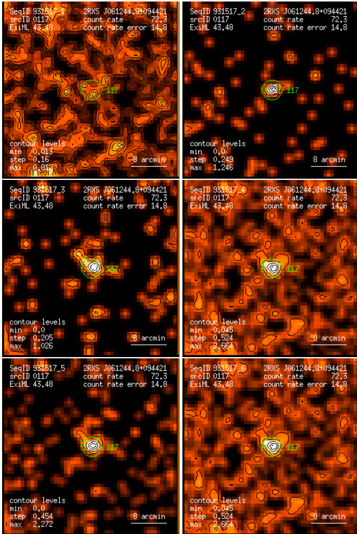
Figure 117: RASS 931517: detection 0117: band rate images, Gaussian filter: (1) PSPC channels 11 – 41, (2) 52 – 90, (3) 91 – 201, (4) 11 – 235, (5) 52 – 201, (6) 11 – 201. Broad band rates in counts/ks. Band rate contour levels in counts/ks/arcmin 2 .
