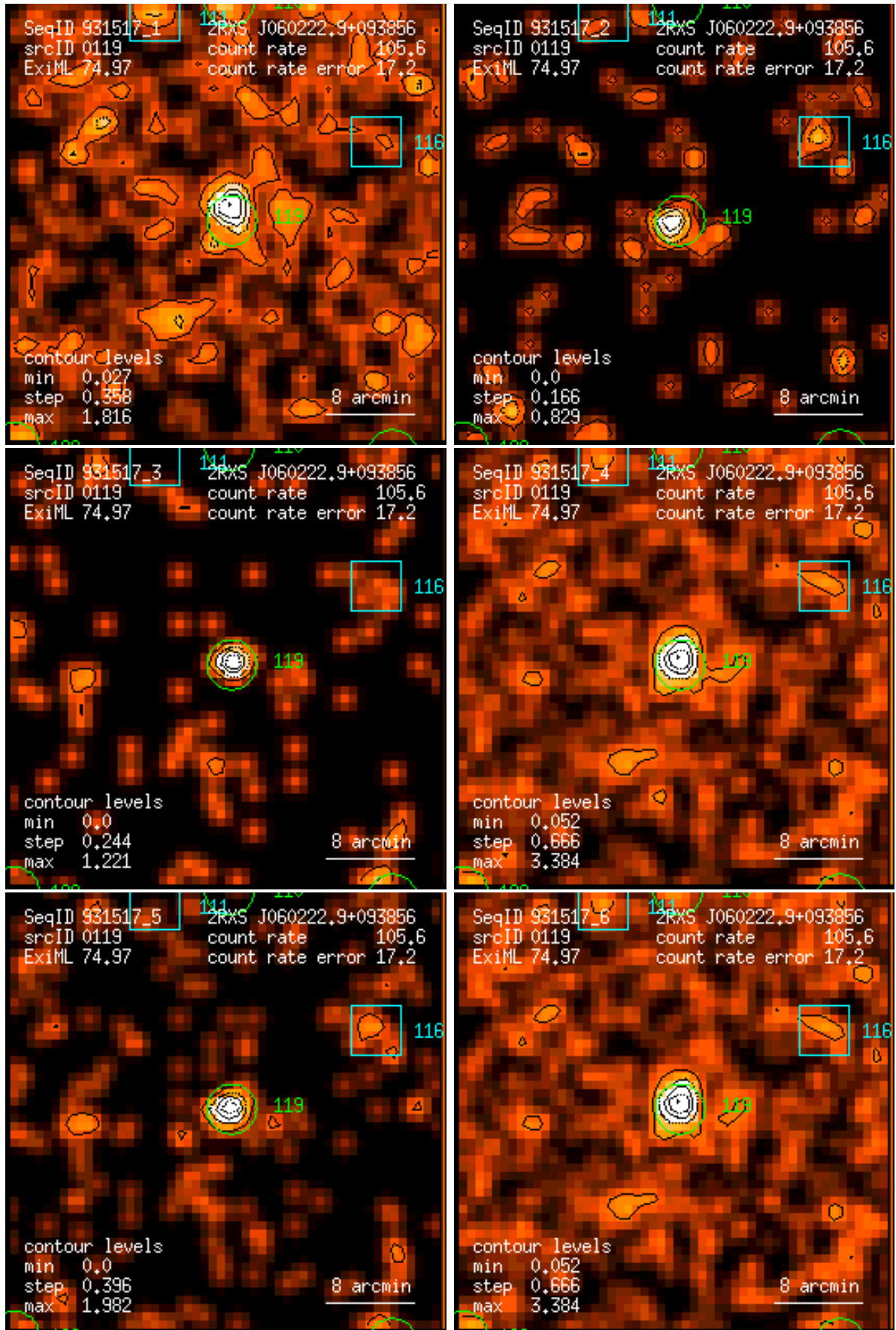
Figure 119: RASS 931517: detection 0119: band rate images, Gaussian filter: (1) PSPC channels 11 – 41, (2) 52 – 90, (3) 91 – 201, (4) 11 – 235, (5) 52 – 201, (6) 11 – 201. Broad band rates in counts/ks. Band rate contour levels in counts/ks/arcmin 2 .
