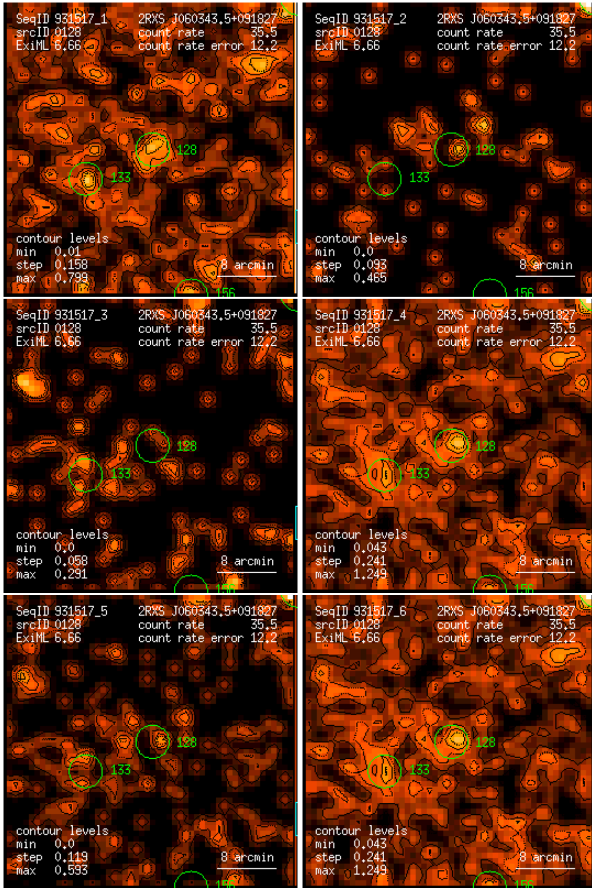
Figure 128: RASS 931517: detection 0128: band rate images, Gaussian filter: (1) PSPC channels 11 – 41, (2) 52 – 90, (3) 91 – 201, (4) 11 – 235, (5) 52 – 201, (6) 11 – 201. Broad band rates in counts/ks. Band rate contour levels in counts/ks/arcmin 2 .
