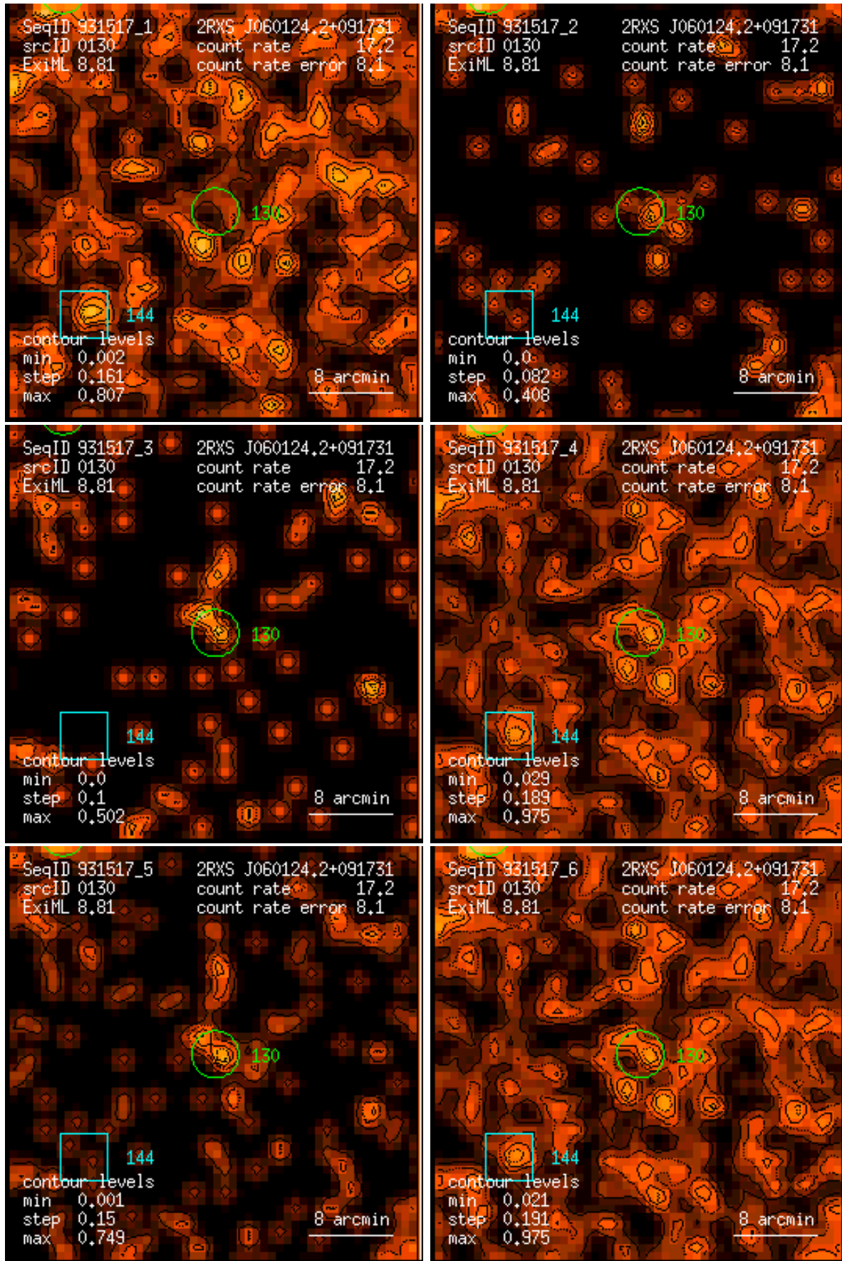
Figure 130: RASS 931517: detection 0130: band rate images, Gaussian filter: (1) PSPC channels 11 – 41, (2) 52 – 90, (3) 91 – 201, (4) 11 – 235, (5) 52 – 201, (6) 11 – 201. Broad band rates in counts/ks. Band rate contour levels in counts/ks/arcmin 2 .
