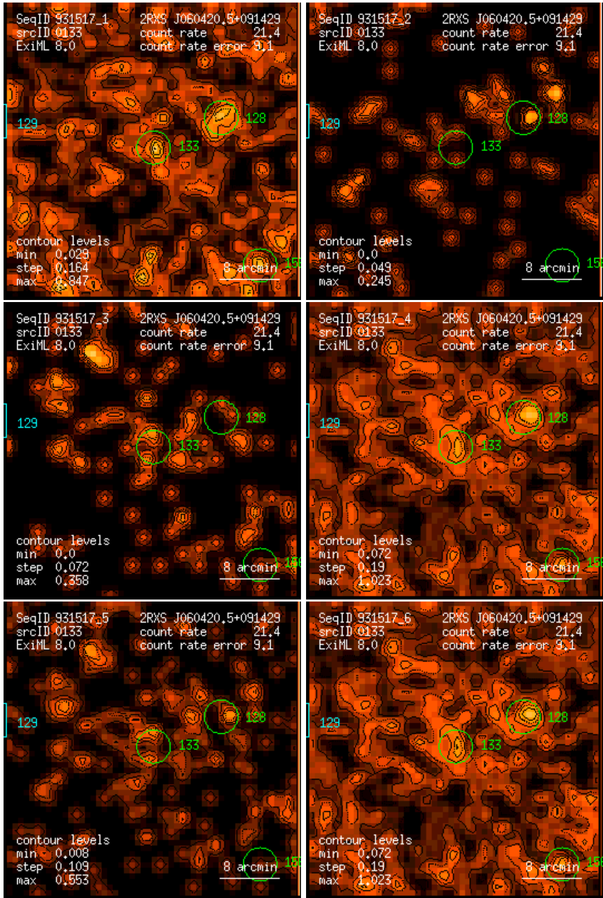
Figure 133: RASS 931517: detection 0133: band rate images, Gaussian filter: (1) PSPC channels 11 – 41, (2) 52 – 90, (3) 91 – 201, (4) 11 – 235, (5) 52 – 201, (6) 11 – 201. Broad band rates in counts/ks. Band rate contour levels in counts/ks/arcmin 2 .
