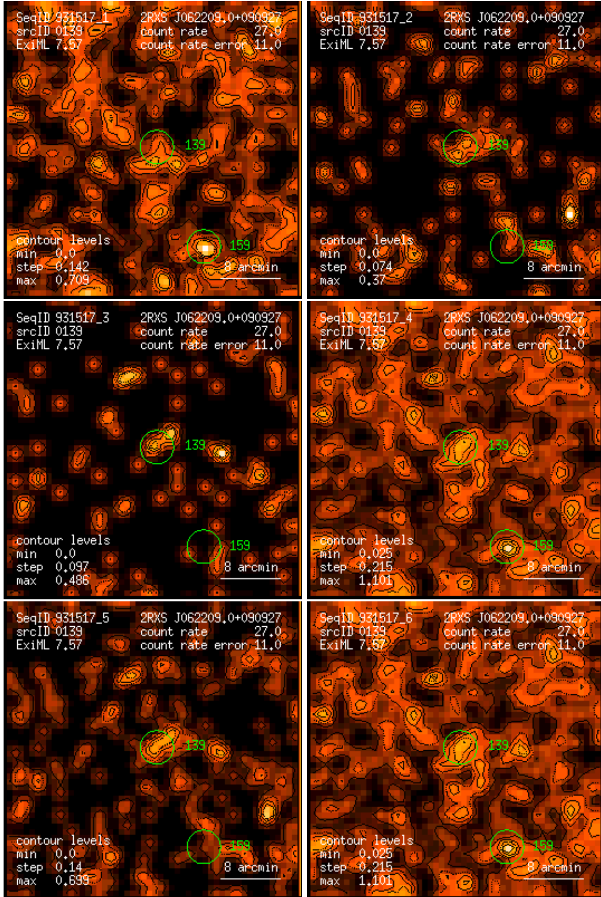
Figure 139: RASS 931517: detection 0139: band rate images, Gaussian filter: (1) PSPC channels 11 – 41, (2) 52 – 90, (3) 91 – 201, (4) 11 – 235, (5) 52 – 201, (6) 11 – 201. Broad band rates in counts/ks. Band rate contour levels in counts/ks/arcmin 2 .
