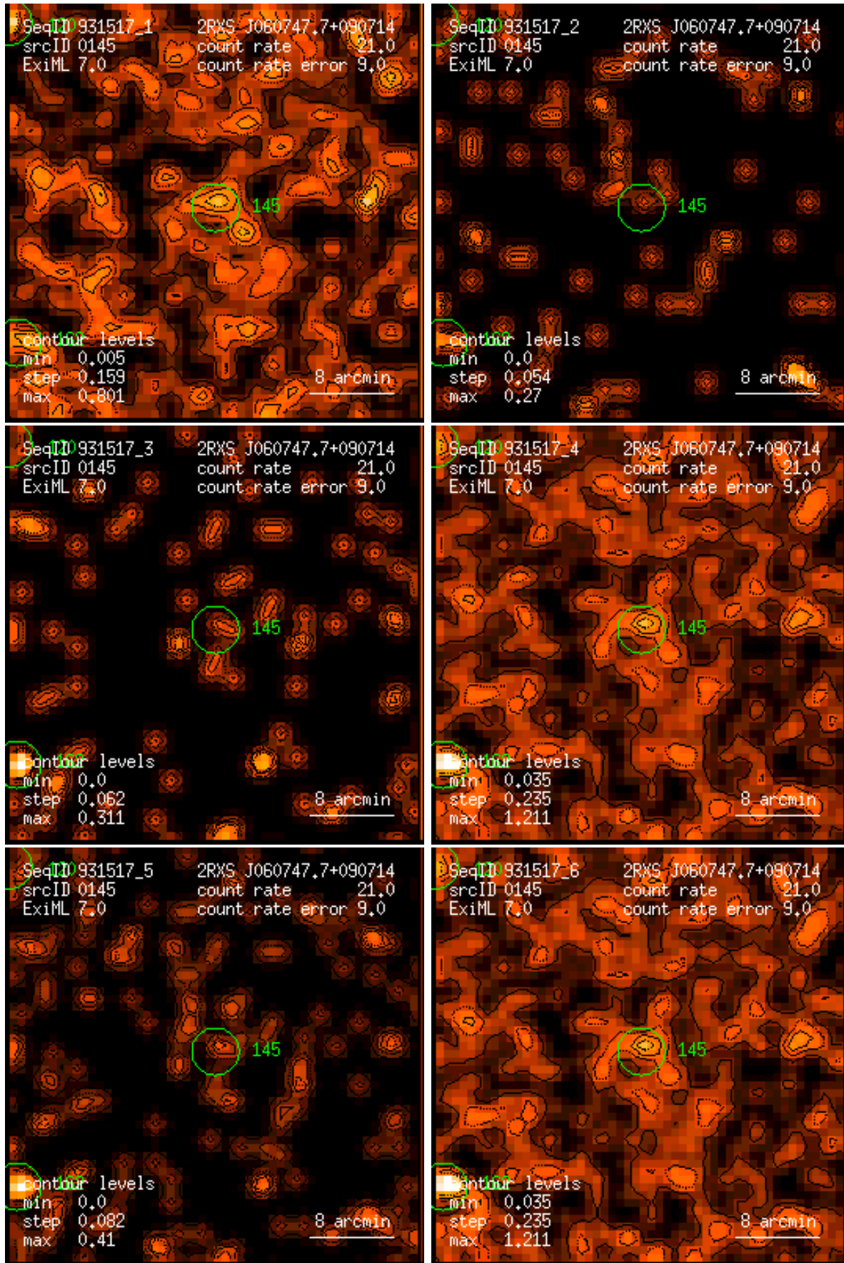
Figure 145: RASS 931517: detection 0145: band rate images, Gaussian filter: (1) PSPC channels 11 – 41, (2) 52 – 90, (3) 91 – 201, (4) 11 – 235, (5) 52 – 201, (6) 11 – 201. Broad band rates in counts/ks. Band rate contour levels in counts/ks/arcmin 2 .
