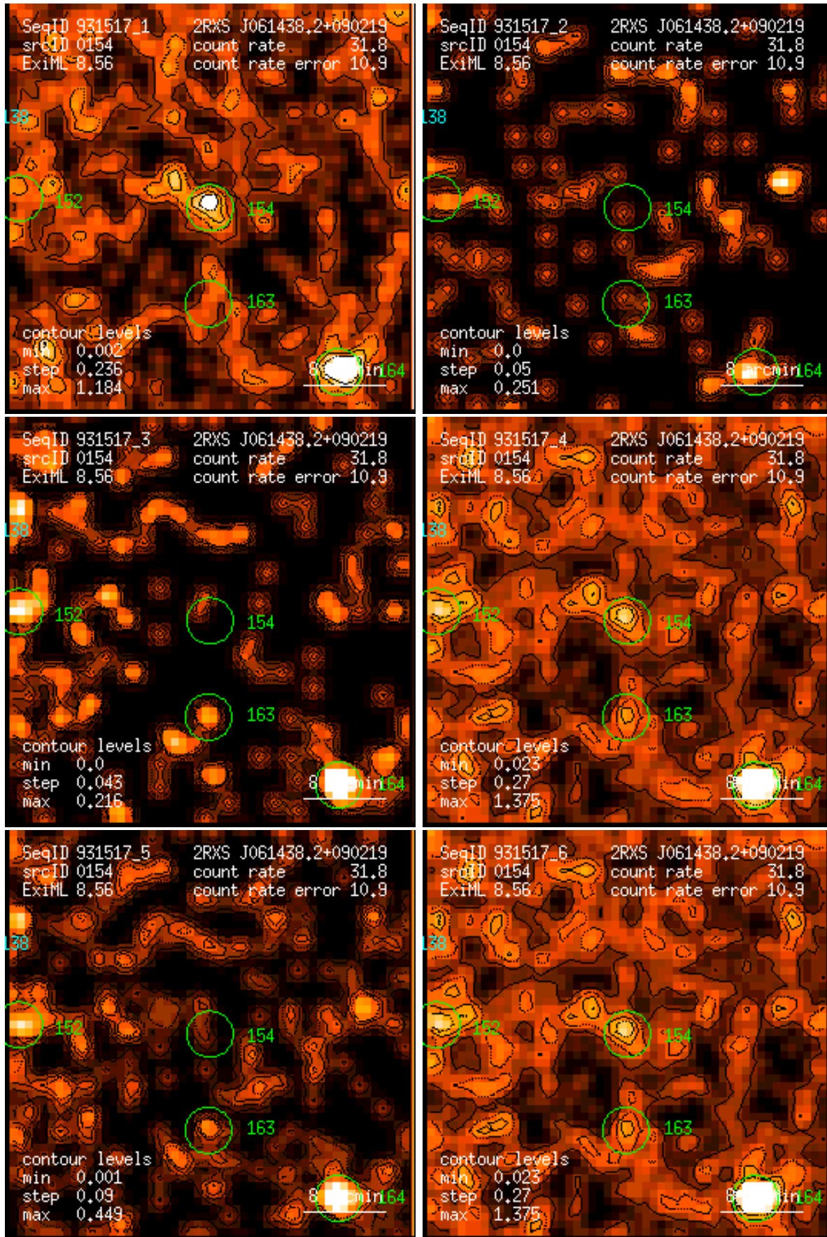
Figure 154: RASS 931517: detection 0154: band rate images, Gaussian filter: (1) PSPC channels 11 – 41, (2) 52 – 90, (3) 91 – 201, (4) 11 – 235, (5) 52 – 201, (6) 11 – 201. Broad band rates in counts/ks. Band rate contour levels in counts/ks/arcmin 2 .
