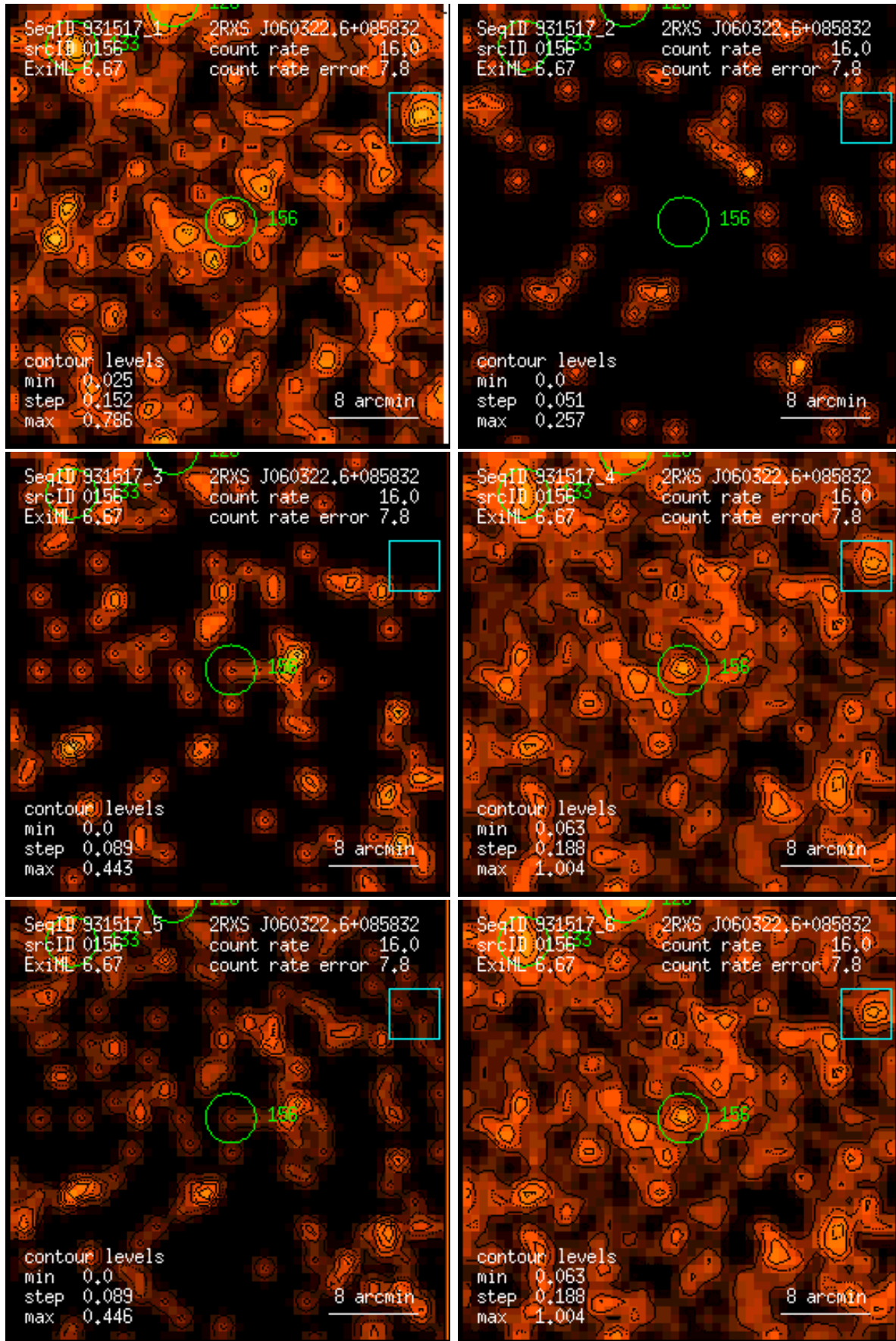
Figure 156: RASS 931517: detection 0156: band rate images, Gaussian filter: (1) PSPC channels 11 – 41, (2) 52 – 90, (3) 91 – 201, (4) 11 – 235, (5) 52 – 201, (6) 11 – 201. Broad band rates in counts/ks. Band rate contour levels in counts/ks/arcmin 2 .
