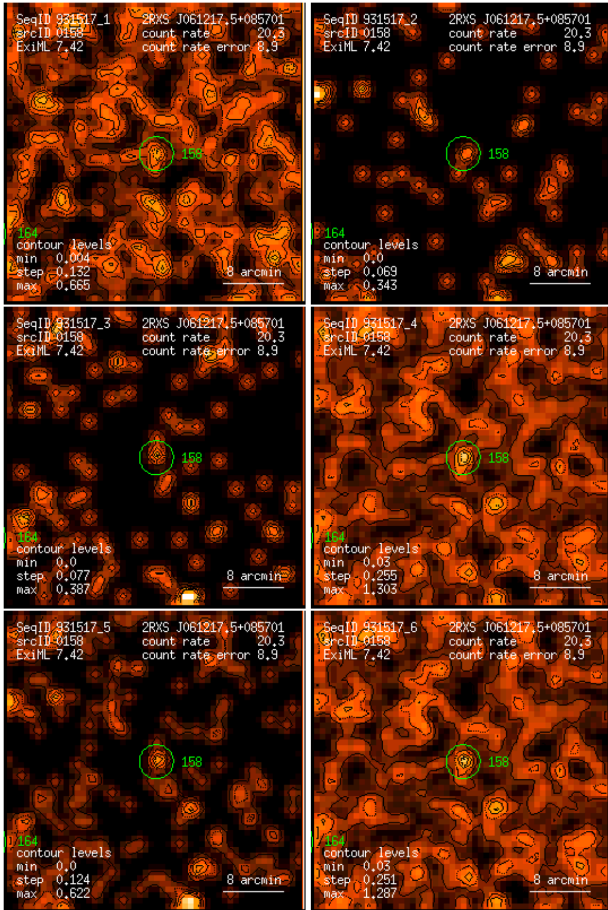
Figure 158: RASS 931517: detection 0158: band rate images, Gaussian filter: (1) PSPC channels 11 – 41, (2) 52 – 90, (3) 91 – 201, (4) 11 – 235, (5) 52 – 201, (6) 11 – 201. Broad band rates in counts/ks. Band rate contour levels in counts/ks/arcmin 2 .
