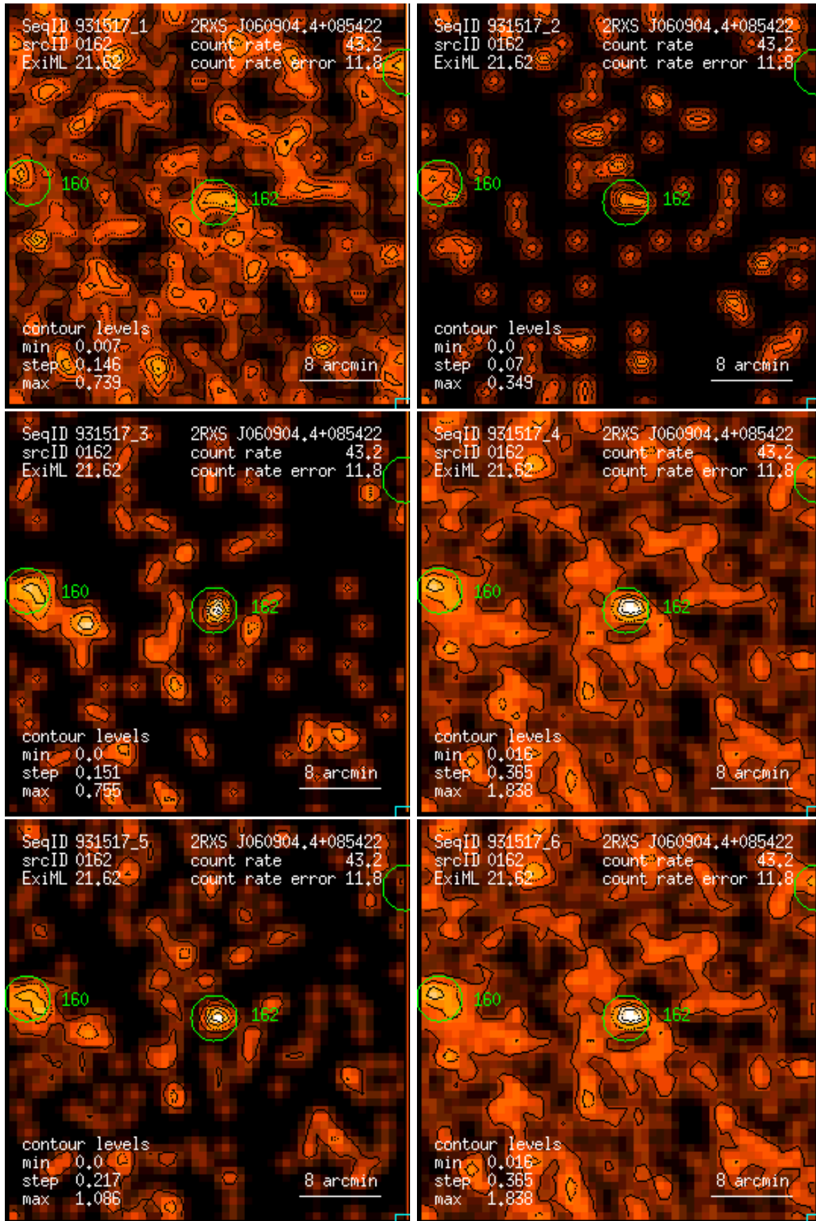
Figure 162: RASS 931517: detection 0162: band rate images, Gaussian filter: (1) PSPC channels 11 – 41, (2) 52 – 90, (3) 91 – 201, (4) 11 – 235, (5) 52 – 201, (6) 11 – 201. Broad band rates in counts/ks. Band rate contour levels in counts/ks/arcmin 2 .
