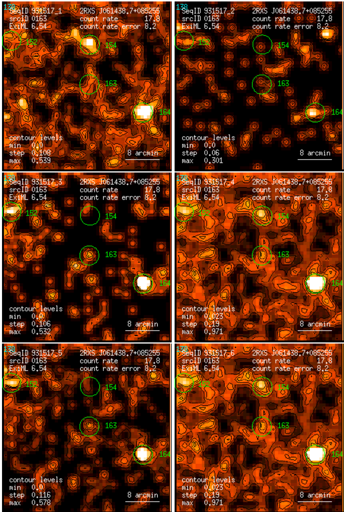
Figure 163: RASS 931517: detection 0163: band rate images, Gaussian filter: (1) PSPC channels 11 – 41, (2) 52 – 90, (3) 91 – 201, (4) 11 – 235, (5) 52 – 201, (6) 11 – 201. Broad band rates in counts/ks. Band rate contour levels in counts/ks/arcmin 2 .
