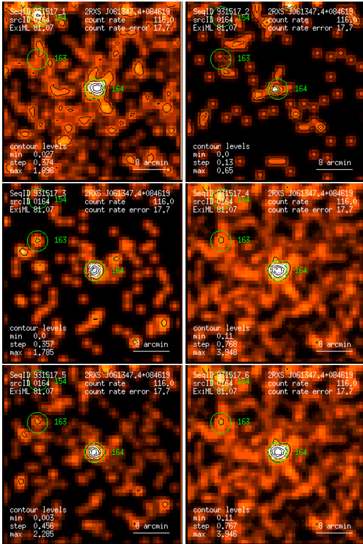
Figure 164: RASS 931517: detection 0164: band rate images, Gaussian filter: (1) PSPC channels 11 – 41, (2) 52 – 90, (3) 91 – 201, (4) 11 – 235, (5) 52 – 201, (6) 11 – 201. Broad band rates in counts/ks. Band rate contour levels in counts/ks/arcmin 2 .
