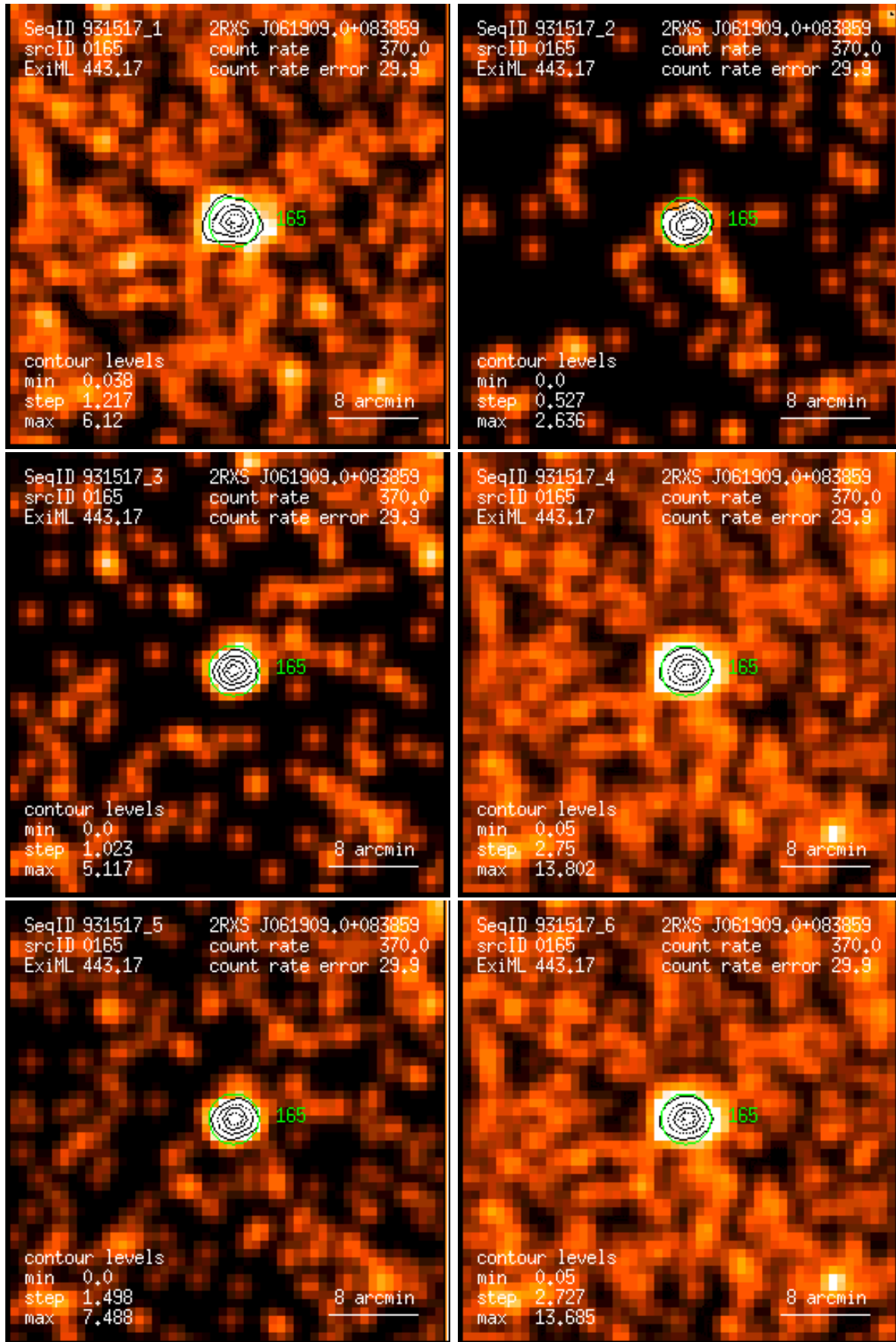
Figure 165: RASS 931517: detection 0165: band rate images, Gaussian filter: (1) PSPC channels 11 – 41, (2) 52 – 90, (3) 91 – 201, (4) 11 – 235, (5) 52 – 201, (6) 11 – 201. Broad band rates in counts/ks. Band rate contour levels in counts/ks/arcmin 2 .
