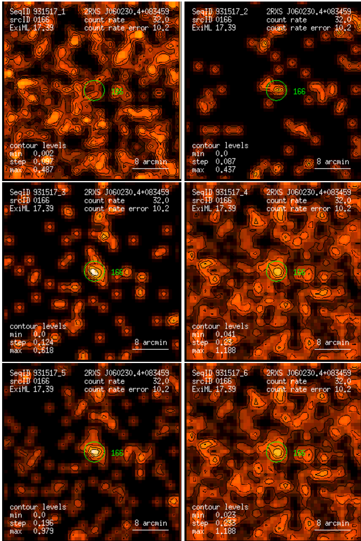
Figure 166: RASS 931517: detection 0166: band rate images, Gaussian filter: (1) PSPC channels 11 – 41, (2) 52 – 90, (3) 91 – 201, (4) 11 – 235, (5) 52 – 201, (6) 11 – 201. Broad band rates in counts/ks. Band rate contour levels in counts/ks/arcmin 2 .
