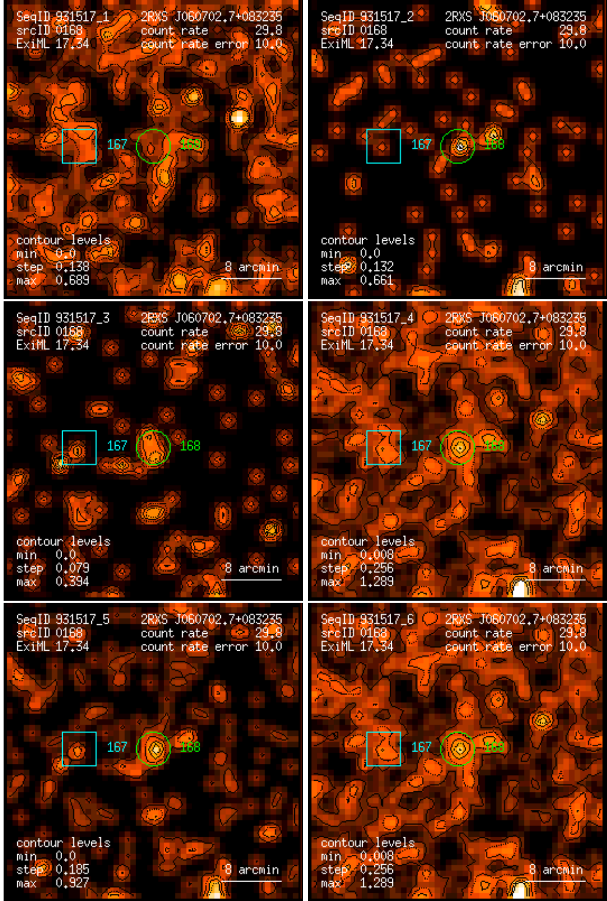
Figure 168: RASS 931517: detection 0168: band rate images, Gaussian filter: (1) PSPC channels 11 – 41, (2) 52 – 90, (3) 91 – 201, (4) 11 – 235, (5) 52 – 201, (6) 11 – 201. Broad band rates in counts/ks. Band rate contour levels in counts/ks/arcmin 2 .
