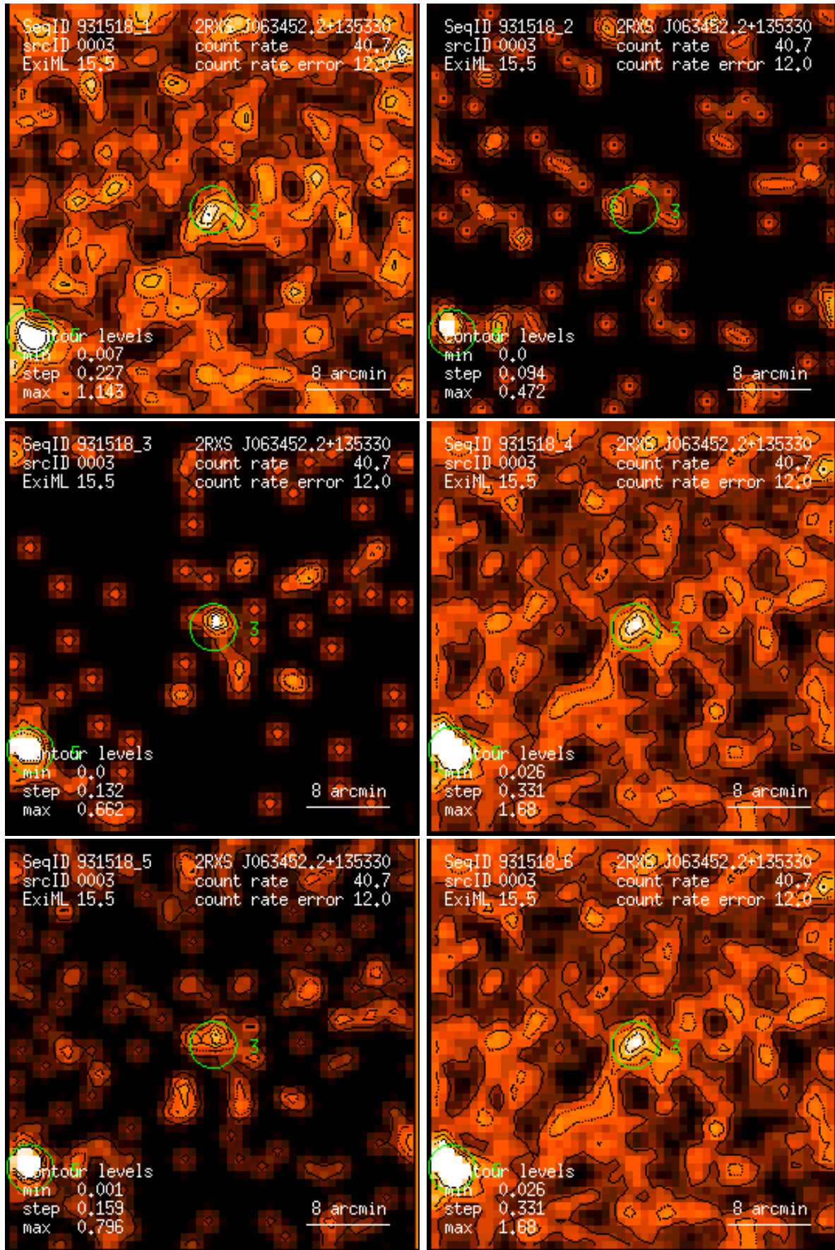
Figure 3: RASS 931518: detection 0003: band rate images, Gaussian filter: (1) PSPC channels 11 – 41, (2) 52 – 90, (3) 91 – 201, (4) 11 – 235, (5) 52 – 201, (6) 11 – 201. Broad band rates in counts/ks. Band rate contour levels in counts/ks/arcmin 2 .
