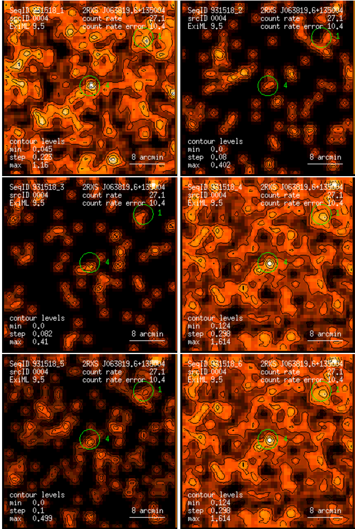
Figure 4: RASS 931518: detection 0004: band rate images, Gaussian filter: (1) PSPC channels 11 – 41, (2) 52 – 90, (3) 91 – 201, (4) 11 – 235, (5) 52 – 201, (6) 11 – 201. Broad band rates in counts/ks. Band rate contour levels in counts/ks/arcmin 2 .
