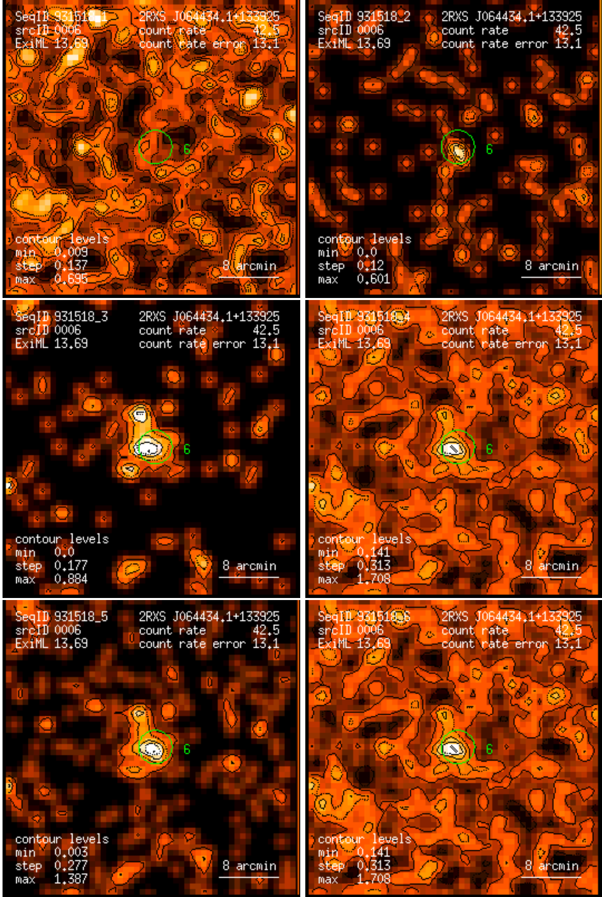
Figure 6: RASS 931518: detection 0006: band rate images, Gaussian filter: (1) PSPC channels 11 – 41, (2) 52 – 90, (3) 91 – 201, (4) 11 – 235, (5) 52 – 201, (6) 11 – 201. Broad band rates in counts/ks. Band rate contour levels in counts/ks/arcmin 2 .
