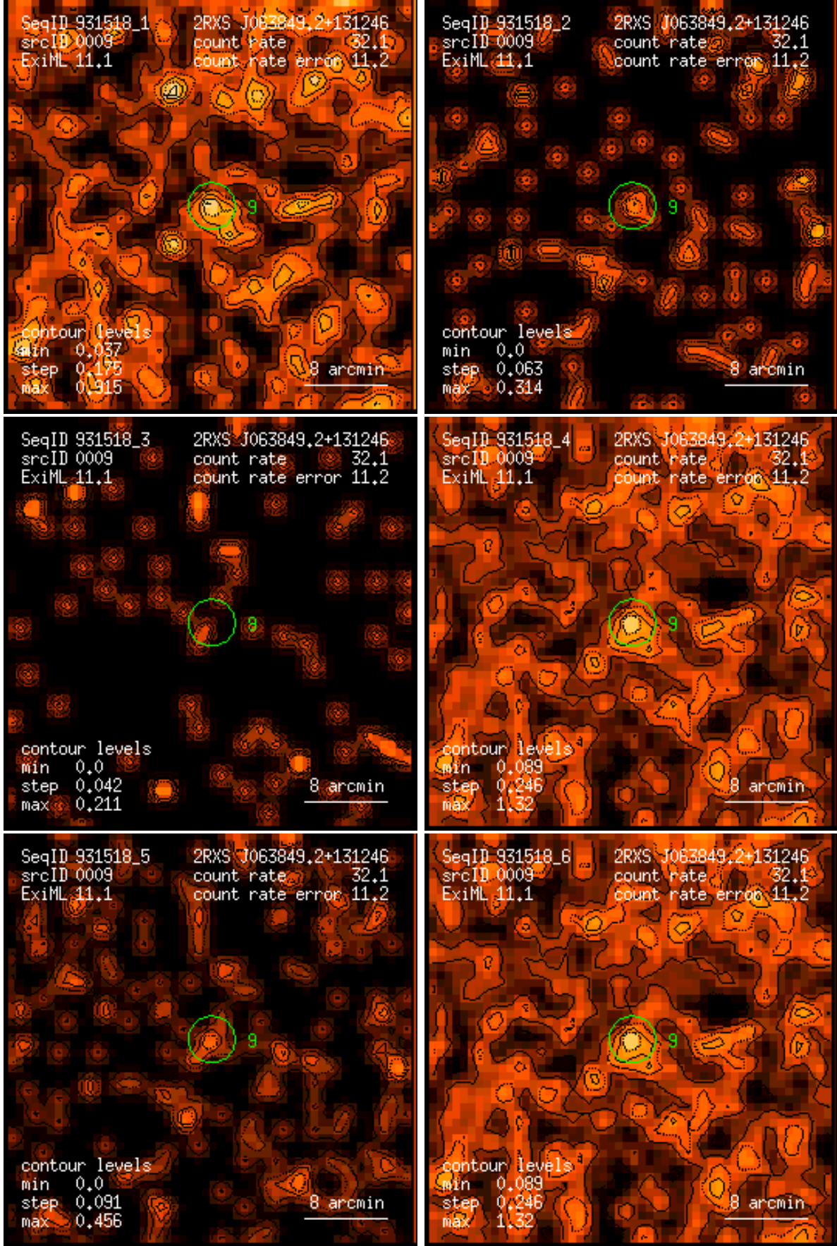
Figure 9: RASS 931518: detection 0009: band rate images, Gaussian filter: (1) PSPC channels 11 – 41, (2) 52 – 90, (3) 91 – 201, (4) 11 – 235, (5) 52 – 201, (6) 11 – 201. Broad band rates in counts/ks. Band rate contour levels in counts/ks/arcmin 2 .
