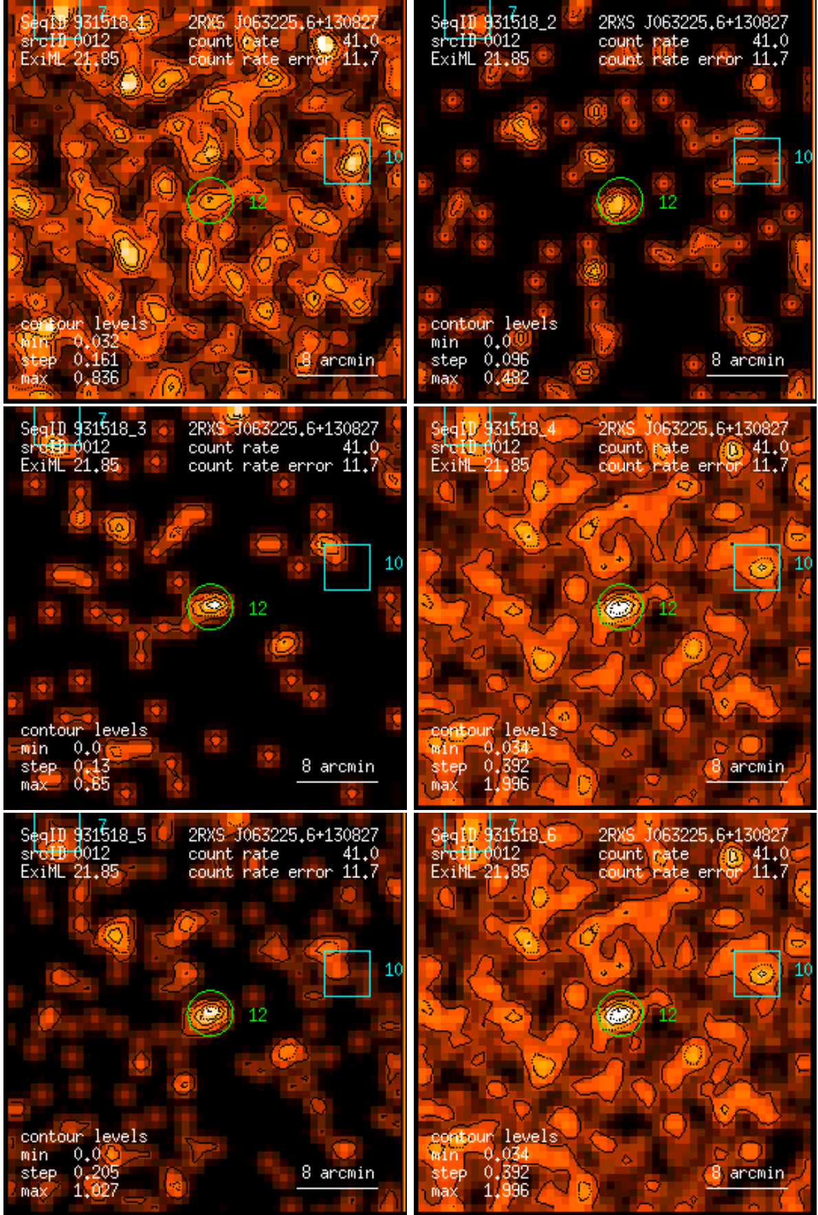
Figure 12: RASS 931518: detection 0012: band rate images, Gaussian filter: (1) PSPC channels 11 – 41, (2) 52 – 90, (3) 91 – 201, (4) 11 – 235, (5) 52 – 201, (6) 11 – 201. Broad band rates in counts/ks. Band rate contour levels in counts/ks/arcmin 2 .
