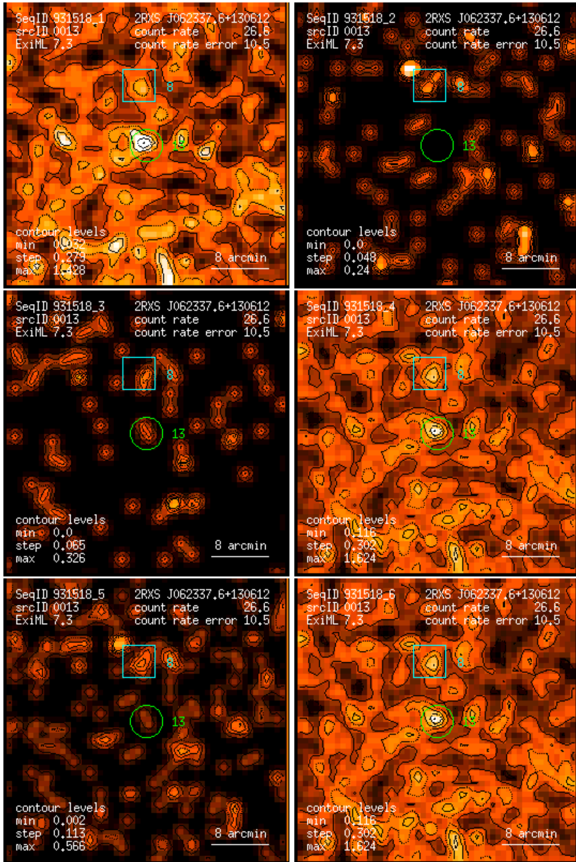
Figure 13: RASS 931518: detection 0013: band rate images, Gaussian filter: (1) PSPC channels 11 – 41, (2) 52 – 90, (3) 91 – 201, (4) 11 – 235, (5) 52 – 201, (6) 11 – 201. Broad band rates in counts/ks. Band rate contour levels in counts/ks/arcmin 2 .
