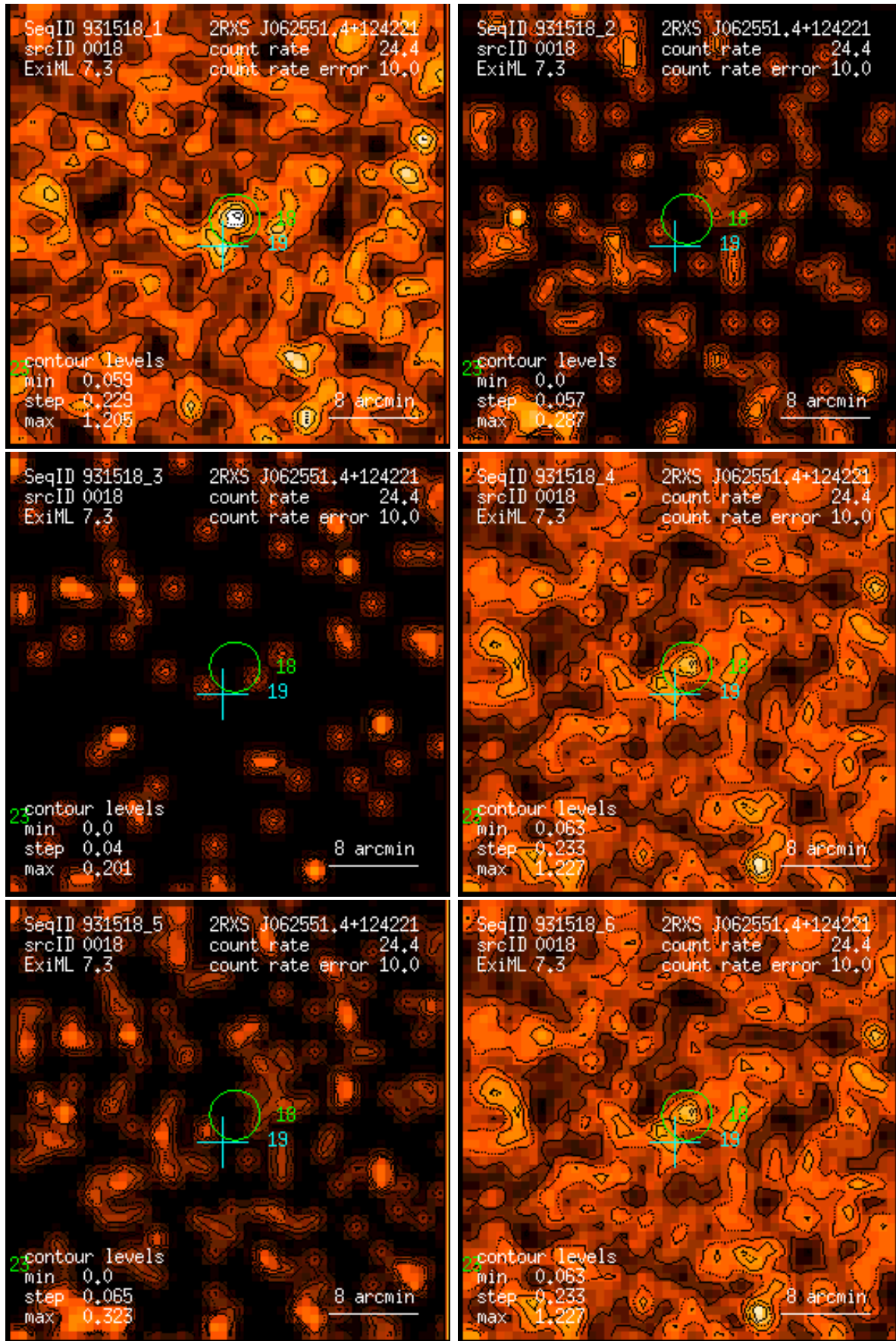
Figure 18: RASS 931518: detection 0018: band rate images, Gaussian filter: (1) PSPC channels 11 – 41, (2) 52 – 90, (3) 91 – 201, (4) 11 – 235, (5) 52 – 201, (6) 11 – 201. Broad band rates in counts/ks. Band rate contour levels in counts/ks/arcmin 2 .
