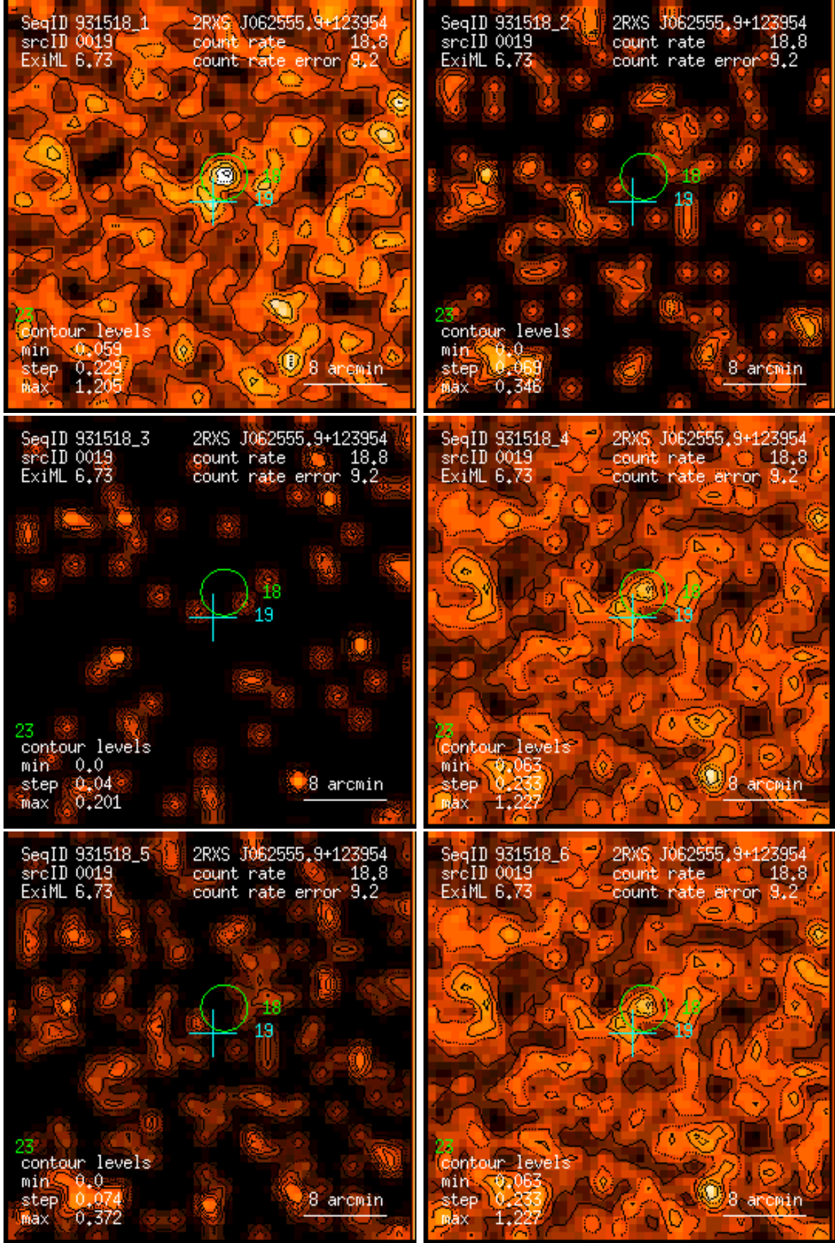
Figure 19: RASS 931518: detection 0019: band rate images, Gaussian filter: (1) PSPC channels 11 – 41, (2) 52 – 90, (3) 91 – 201, (4) 11 – 235, (5) 52 – 201, (6) 11 – 201. Broad band rates in counts/ks. Band rate contour levels in counts/ks/arcmin 2 .
