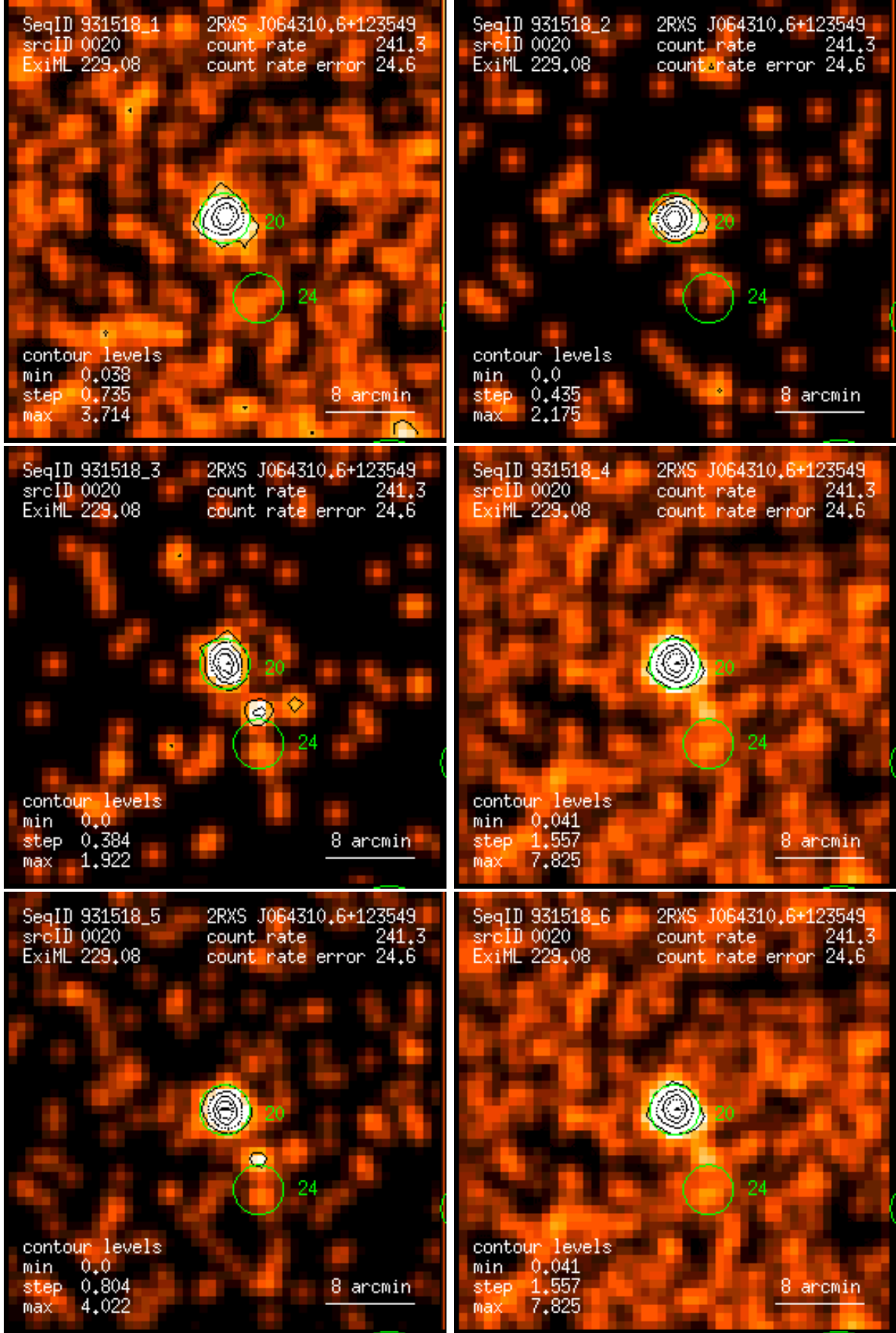
Figure 20: RASS 931518: detection 0020: band rate images, Gaussian filter: (1) PSPC channels 11 – 41, (2) 52 – 90, (3) 91 – 201, (4) 11 – 235, (5) 52 – 201, (6) 11 – 201. Broad band rates in counts/ks. Band rate contour levels in counts/ks/arcmin 2 .
