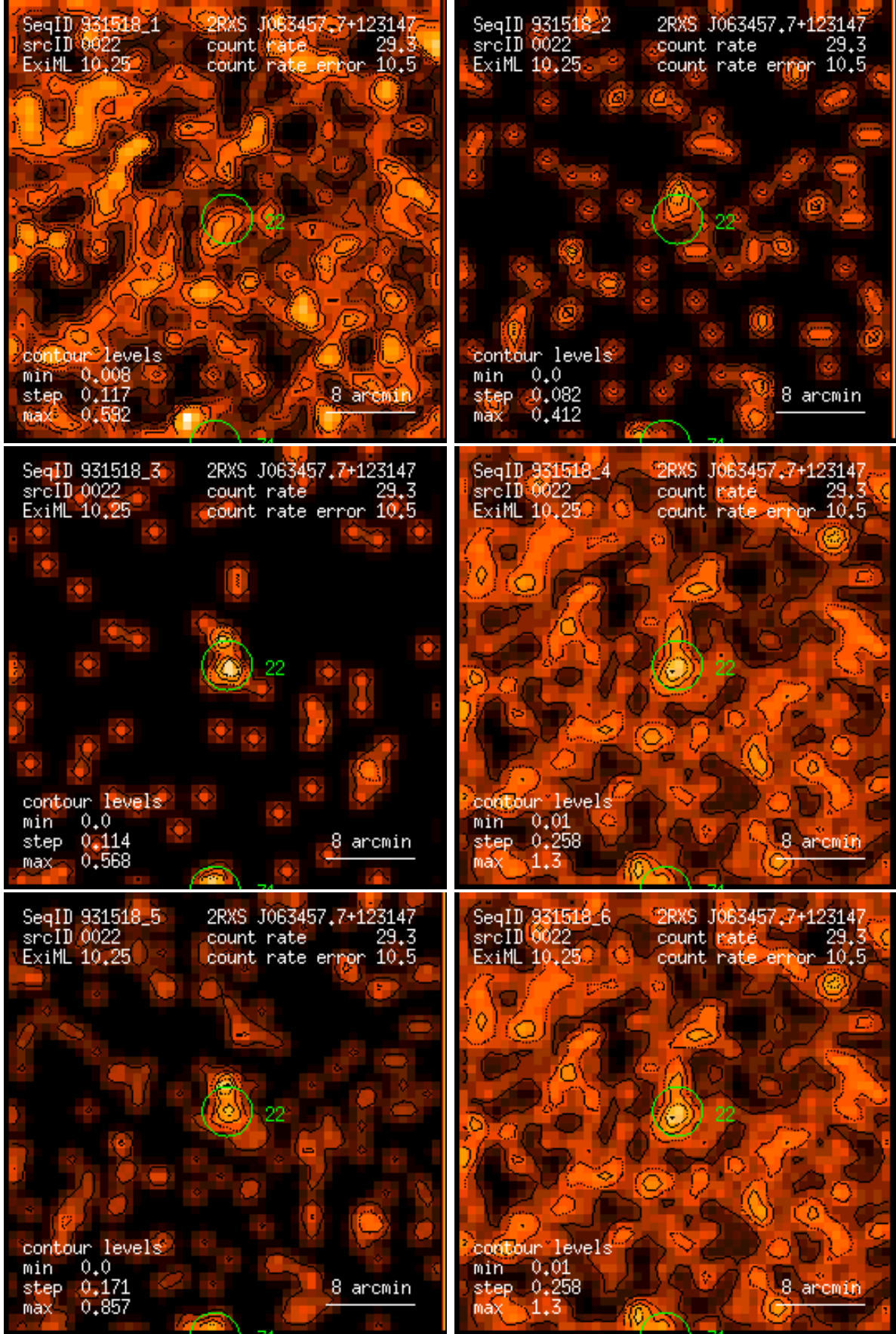
Figure 22: RASS 931518: detection 0022: band rate images, Gaussian filter: (1) PSPC channels 11 – 41, (2) 52 – 90, (3) 91 – 201, (4) 11 – 235, (5) 52 – 201, (6) 11 – 201. Broad band rates in counts/ks. Band rate contour levels in counts/ks/arcmin 2 .
