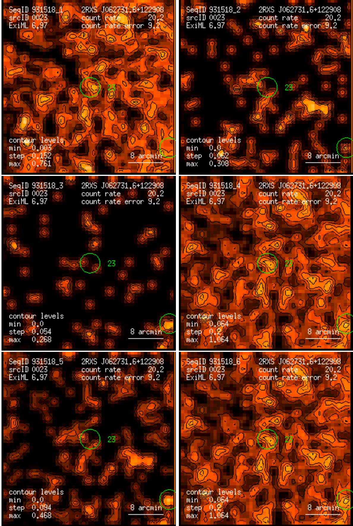
Figure 23: RASS 931518: detection 0023: band rate images, Gaussian filter: (1) PSPC channels 11 – 41, (2) 52 – 90, (3) 91 – 201, (4) 11 – 235, (5) 52 – 201, (6) 11 – 201. Broad band rates in counts/ks. Band rate contour levels in counts/ks/arcmin 2 .
