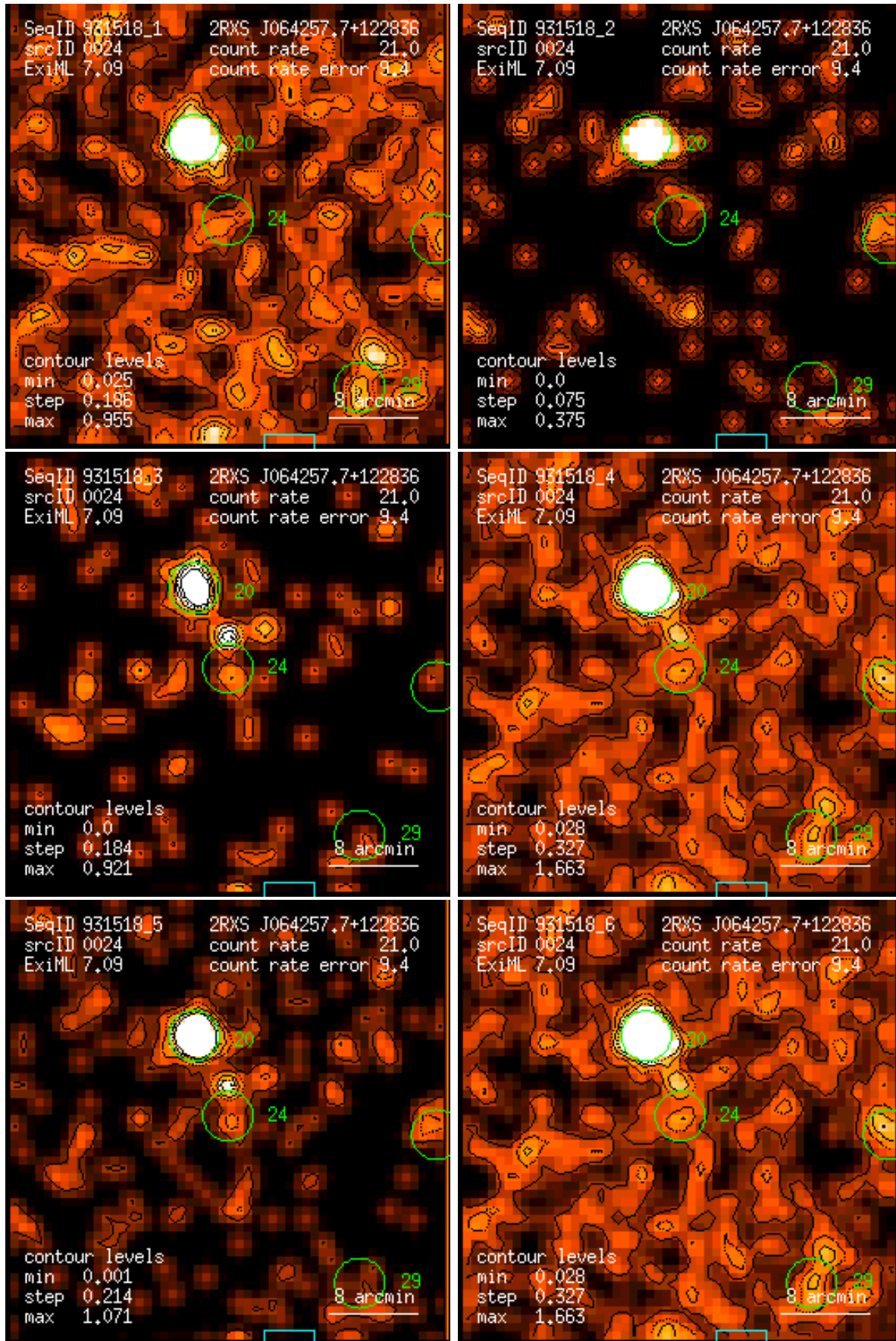
Figure 24: RASS 931518: detection 0024: band rate images, Gaussian filter: (1) PSPC channels 11 – 41, (2) 52 – 90, (3) 91 – 201, (4) 11 – 235, (5) 52 – 201, (6) 11 – 201. Broad band rates in counts/ks. Band rate contour levels in counts/ks/arcmin 2 .
