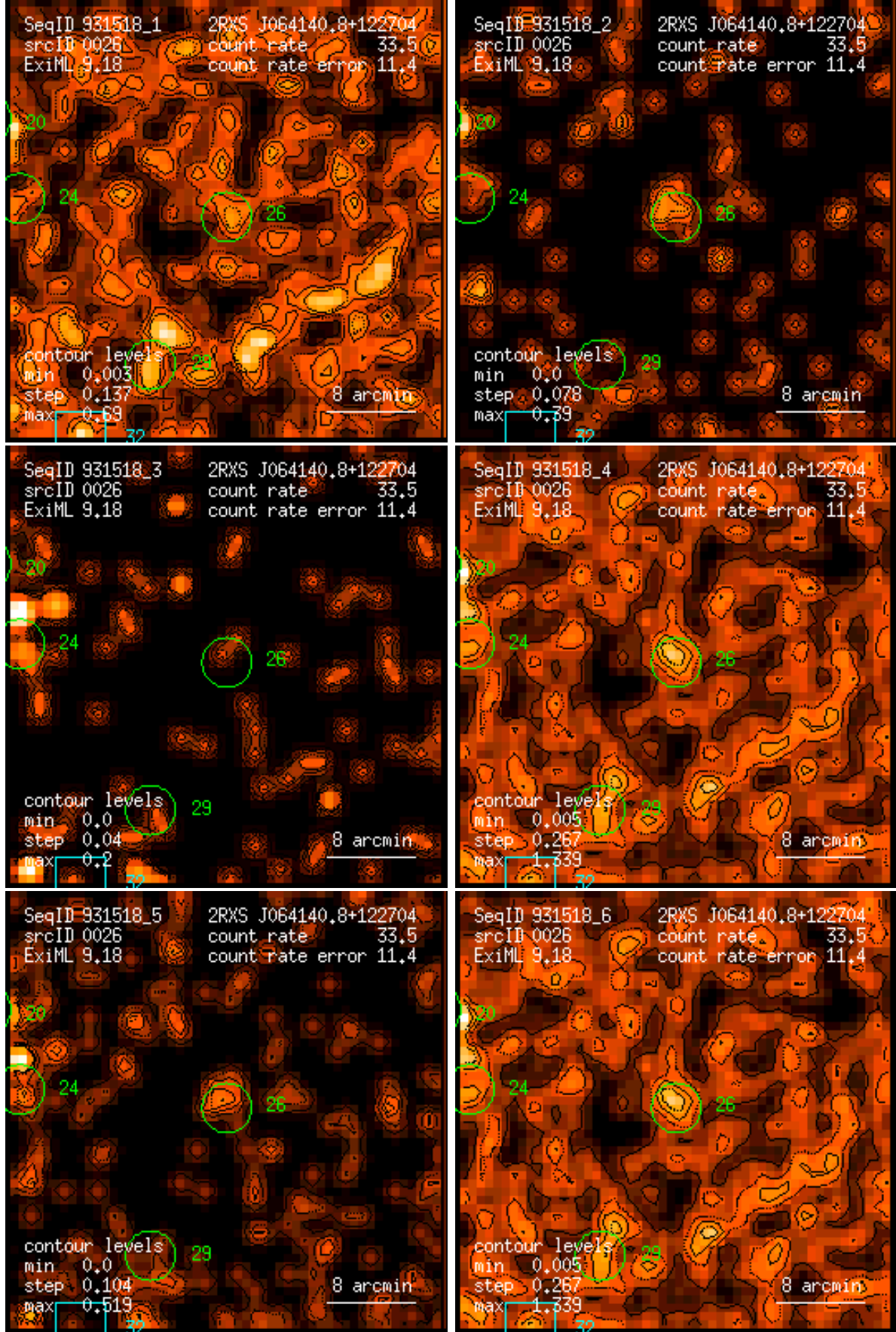
Figure 26: RASS 931518: detection 0026: band rate images, Gaussian filter: (1) PSPC channels 11 – 41, (2) 52 – 90, (3) 91 – 201, (4) 11 – 235, (5) 52 – 201, (6) 11 – 201. Broad band rates in counts/ks. Band rate contour levels in counts/ks/arcmin 2 .
