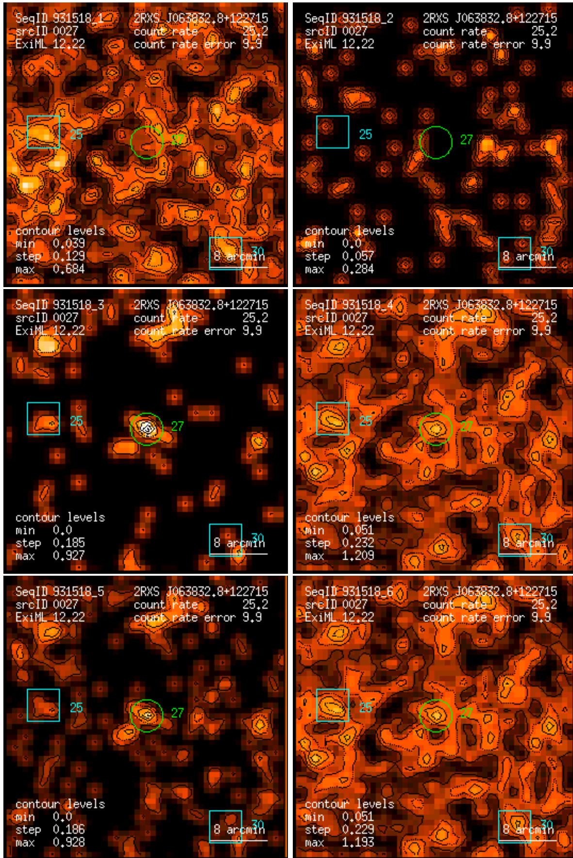
Figure 27: RASS 931518: detection 0027: band rate images, Gaussian filter: (1) PSPC channels 11 – 41, (2) 52 – 90, (3) 91 – 201, (4) 11 – 235, (5) 52 – 201, (6) 11 – 201. Broad band rates in counts/ks. Band rate contour levels in counts/ks/arcmin 2 .
