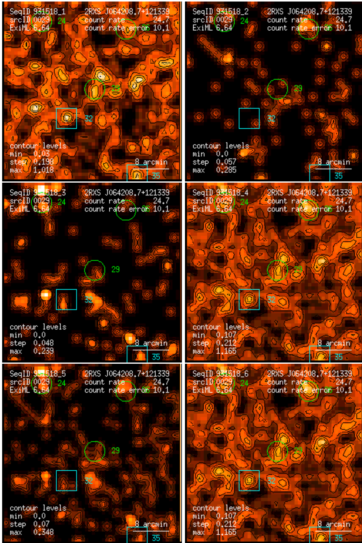
Figure 29: RASS 931518: detection 0029: band rate images, Gaussian filter: (1) PSPC channels 11 – 41, (2) 52 – 90, (3) 91 – 201, (4) 11 – 235, (5) 52 – 201, (6) 11 – 201. Broad band rates in counts/ks. Band rate contour levels in counts/ks/arcmin 2 .
