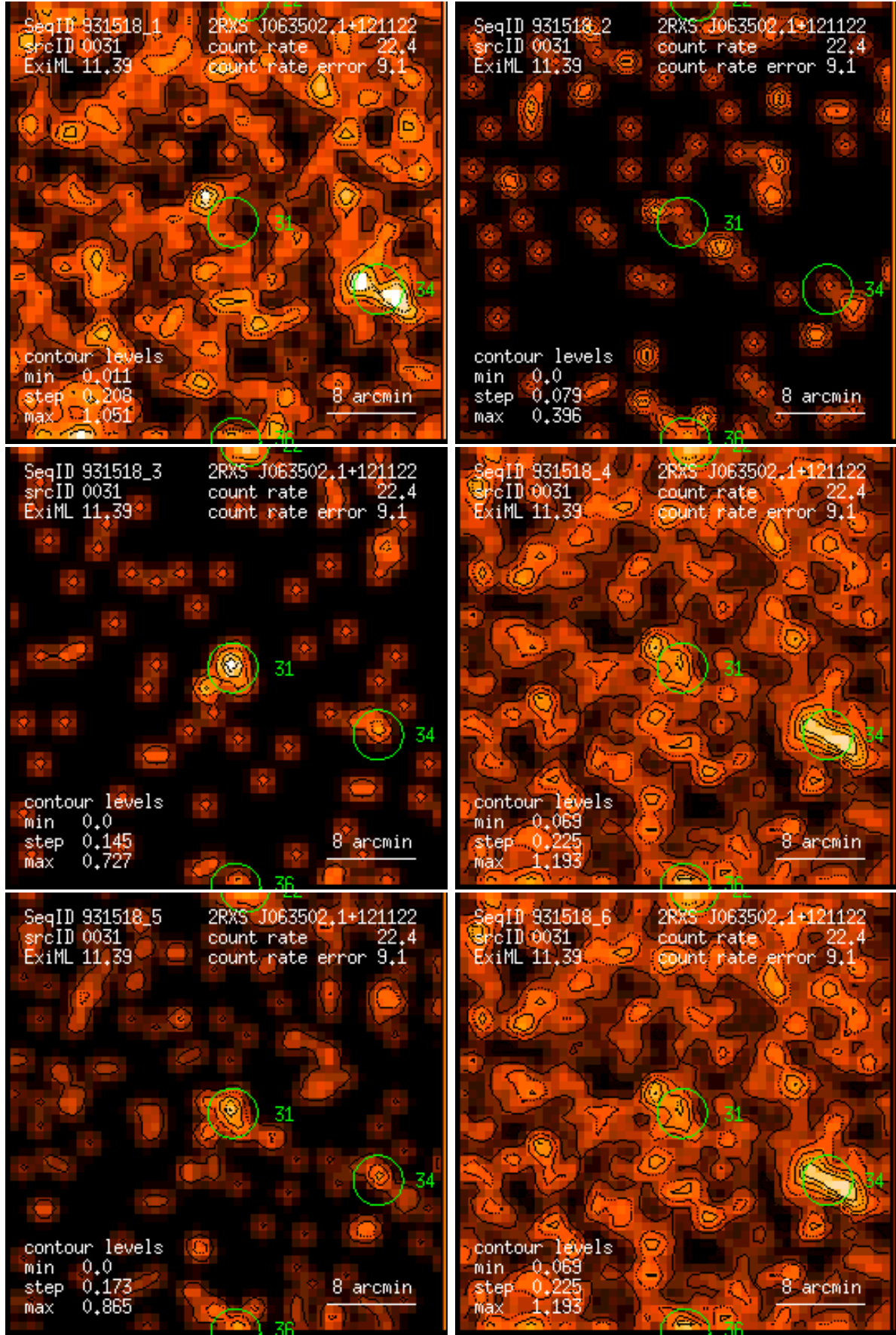
Figure 31: RASS 931518: detection 0031: band rate images, Gaussian filter: (1) PSPC channels 11 – 41, (2) 52 – 90, (3) 91 – 201, (4) 11 – 235, (5) 52 – 201, (6) 11 – 201. Broad band rates in counts/ks. Band rate contour levels in counts/ks/arcmin 2 .
