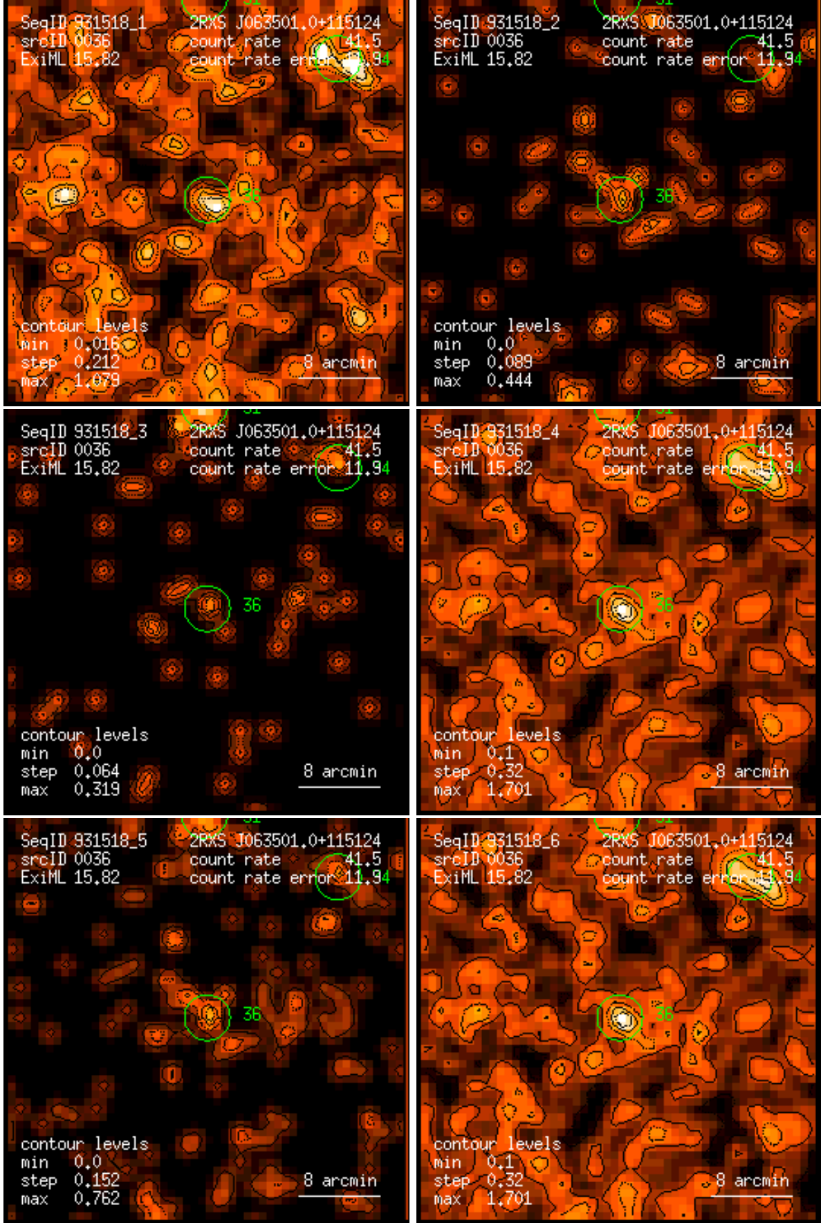
Figure 36: RASS 931518: detection 0036: band rate images, Gaussian filter: (1) PSPC channels 11 – 41, (2) 52 – 90, (3) 91 – 201, (4) 11 – 235, (5) 52 – 201, (6) 11 – 201. Broad band rates in counts/ks. Band rate contour levels in counts/ks/arcmin 2 .
