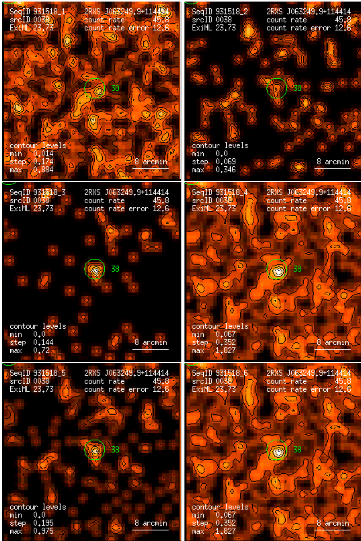
Figure 38: RASS 931518: detection 0038: band rate images, Gaussian filter: (1) PSPC channels 11 – 41, (2) 52 – 90, (3) 91 – 201, (4) 11 – 235, (5) 52 – 201, (6) 11 – 201. Broad band rates in counts/ks. Band rate contour levels in counts/ks/arcmin 2 .
