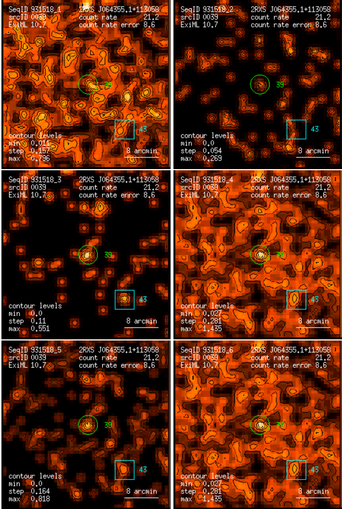
Figure 39: RASS 931518: detection 0039: band rate images, Gaussian filter: (1) PSPC channels 11 – 41, (2) 52 – 90, (3) 91 – 201, (4) 11 – 235, (5) 52 – 201, (6) 11 – 201. Broad band rates in counts/ks. Band rate contour levels in counts/ks/arcmin 2 .
