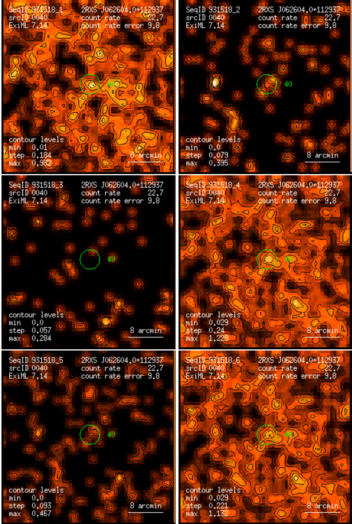
Figure 40: RASS 931518: detection 0040: band rate images, Gaussian filter: (1) PSPC channels 11 – 41, (2) 52 – 90, (3) 91 – 201, (4) 11 – 235, (5) 52 – 201, (6) 11 – 201. Broad band rates in counts/ks. Band rate contour levels in counts/ks/arcmin 2 .
