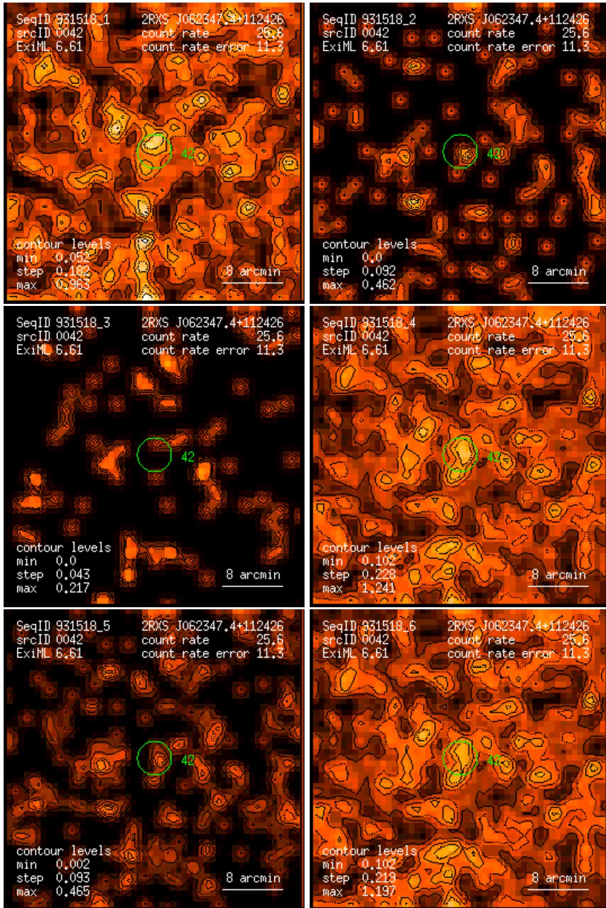
Figure 42: RASS 931518: detection 0042: band rate images, Gaussian filter: (1) PSPC channels 11 – 41, (2) 52 – 90, (3) 91 – 201, (4) 11 – 235, (5) 52 – 201, (6) 11 – 201. Broad band rates in counts/ks. Band rate contour levels in counts/ks/arcmin 2 .
