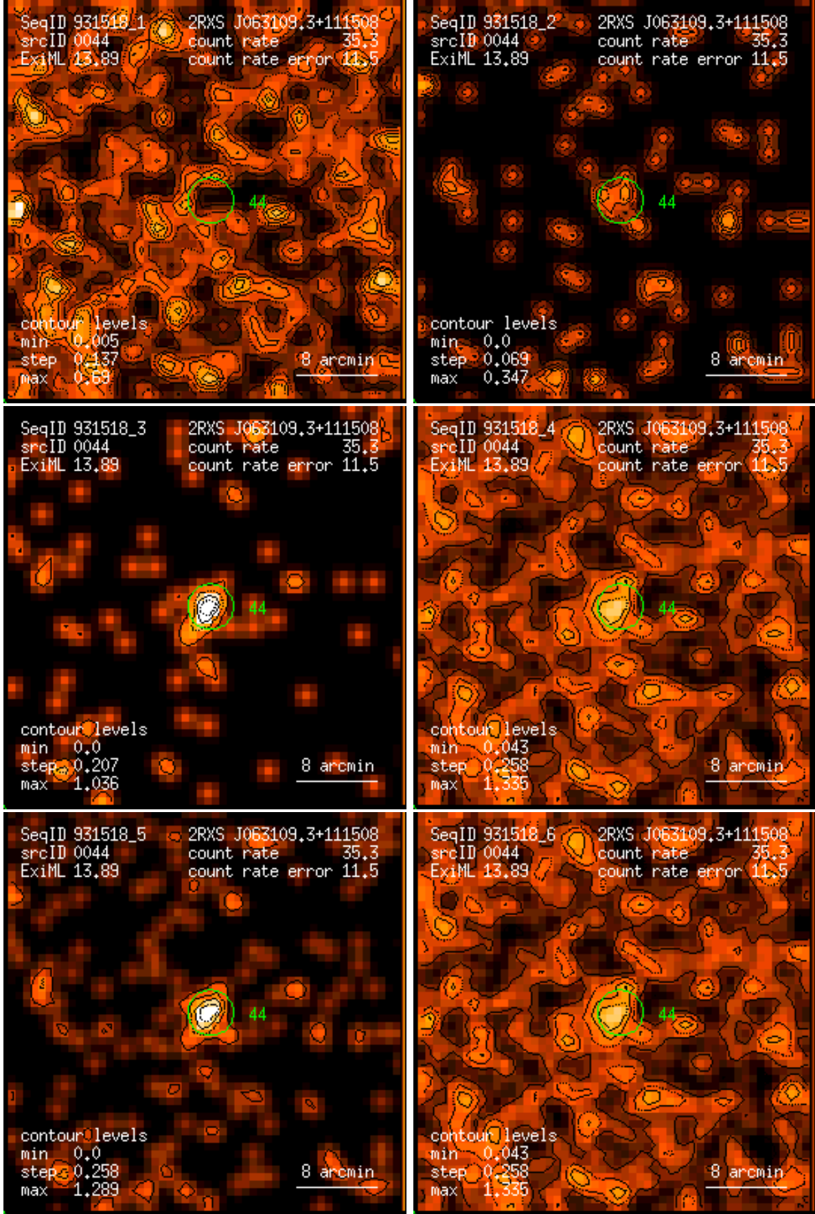
Figure 44: RASS 931518: detection 0044: band rate images, Gaussian filter: (1) PSPC channels 11 – 41, (2) 52 – 90, (3) 91 – 201, (4) 11 – 235, (5) 52 – 201, (6) 11 – 201. Broad band rates in counts/ks. Band rate contour levels in counts/ks/arcmin 2 .
