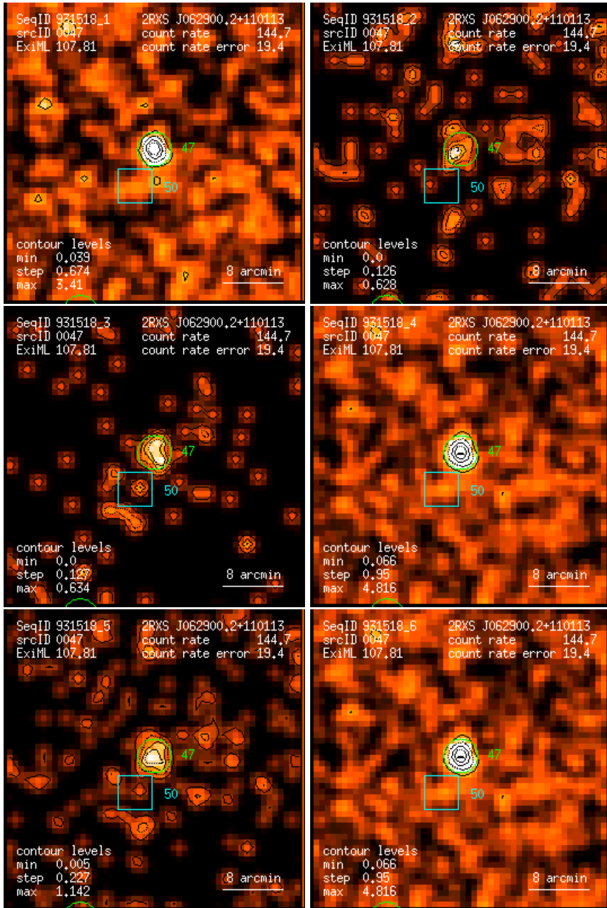
Figure 47: RASS 931518: detection 0047: band rate images, Gaussian filter: (1) PSPC channels 11 – 41, (2) 52 – 90, (3) 91 – 201, (4) 11 – 235, (5) 52 – 201, (6) 11 – 201. Broad band rates in counts/ks. Band rate contour levels in counts/ks/arcmin 2 .
