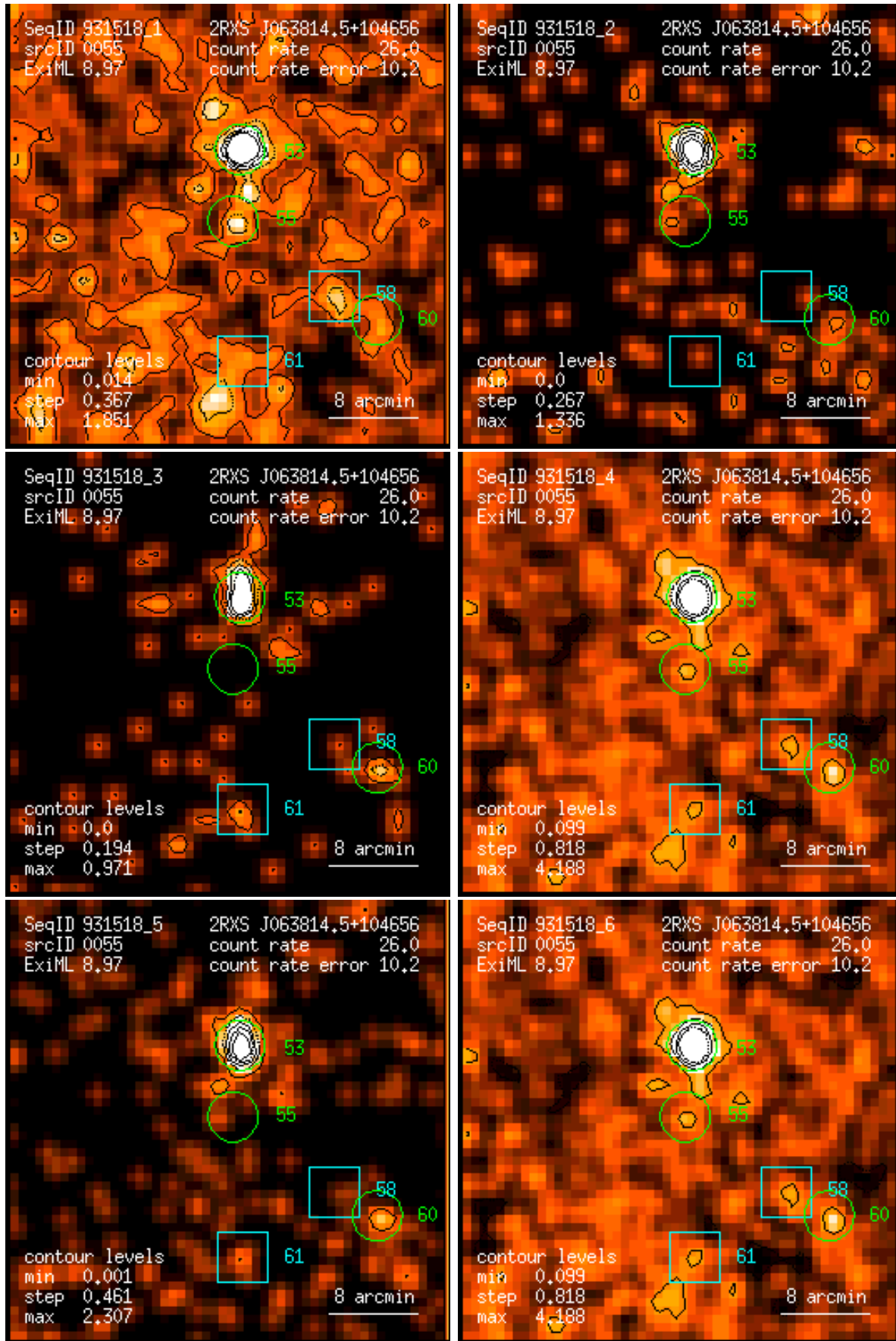
Figure 55: RASS 931518: detection 0055: band rate images, Gaussian filter: (1) PSPC channels 11 – 41, (2) 52 – 90, (3) 91 – 201, (4) 11 – 235, (5) 52 – 201, (6) 11 – 201. Broad band rates in counts/ks. Band rate contour levels in counts/ks/arcmin 2 .
