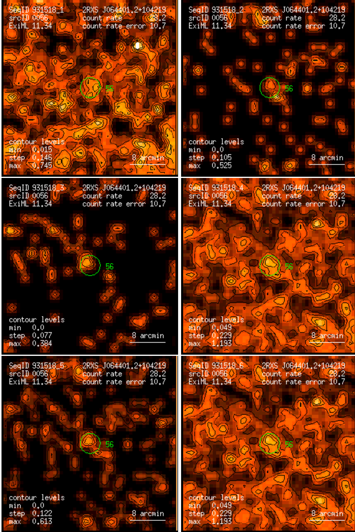
Figure 56: RASS 931518: detection 0056: band rate images, Gaussian filter: (1) PSPC channels 11 – 41, (2) 52 – 90, (3) 91 – 201, (4) 11 – 235, (5) 52 – 201, (6) 11 – 201. Broad band rates in counts/ks. Band rate contour levels in counts/ks/arcmin 2 .
