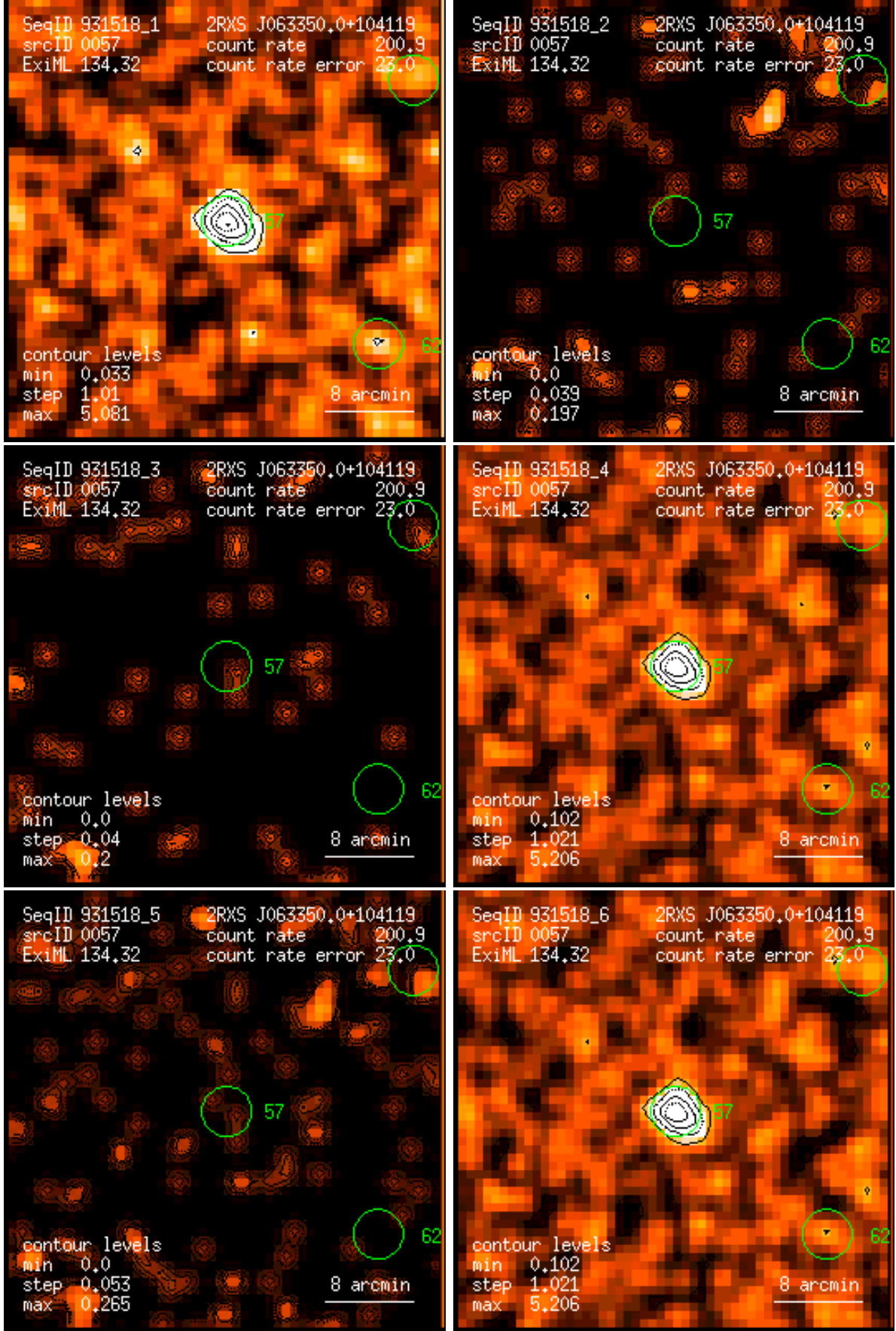
Figure 57: RASS 931518: detection 0057: band rate images, Gaussian filter: (1) PSPC channels 11 – 41, (2) 52 – 90, (3) 91 – 201, (4) 11 – 235, (5) 52 – 201, (6) 11 – 201. Broad band rates in counts/ks. Band rate contour levels in counts/ks/arcmin 2 .
